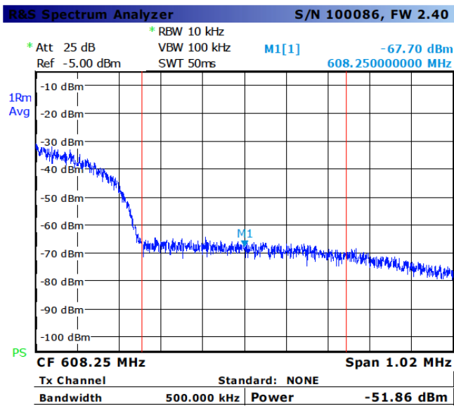
Figure 4—Upper DTV Emission Shoulder
