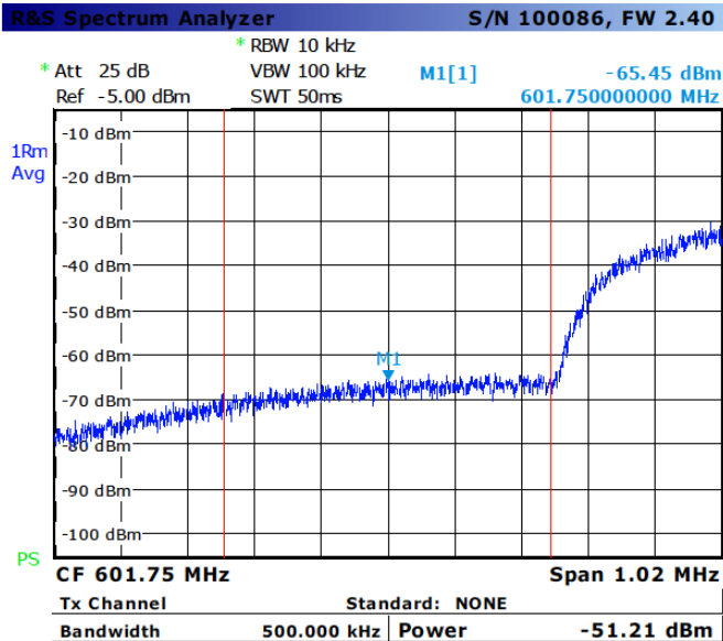
Figure 5—Lower DTV Emission Shoulder
