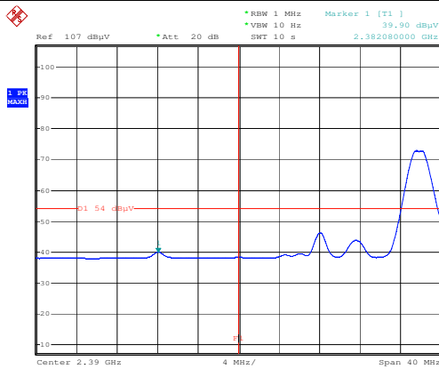
Peak - Left Side-V
