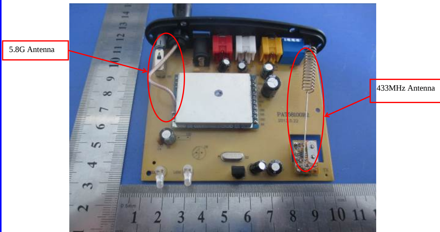
EUT (Receiver)–PCB 1 Front View
