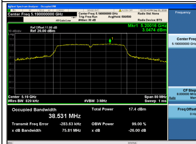
5150-5250MHz Bandwidth - Low CH 5190 (Antenna 2)
