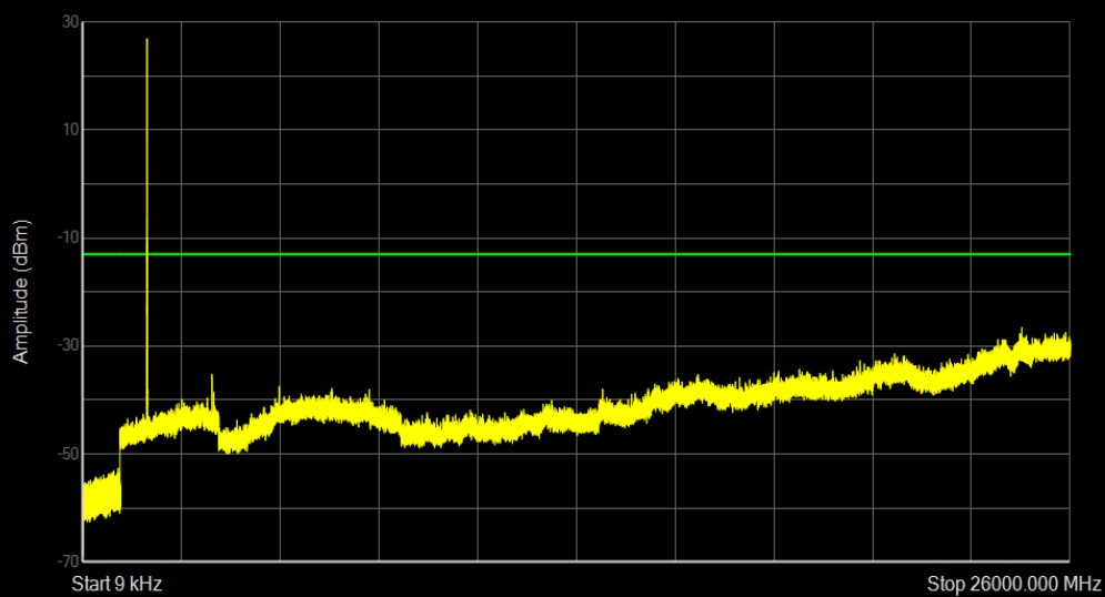
Band66 16QAM BW=20MHz Channel=132572 RB Size=1 Position=#0
