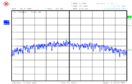
Low -13.01dBm/3kHz
