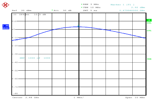
High 2.92dBm
