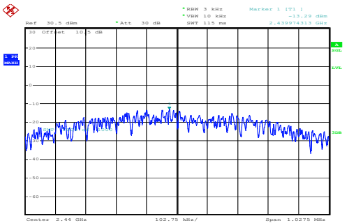
Middle -13.29dBm/3kHz
