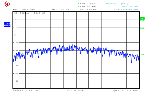
High -13.00dBm/3kHz
