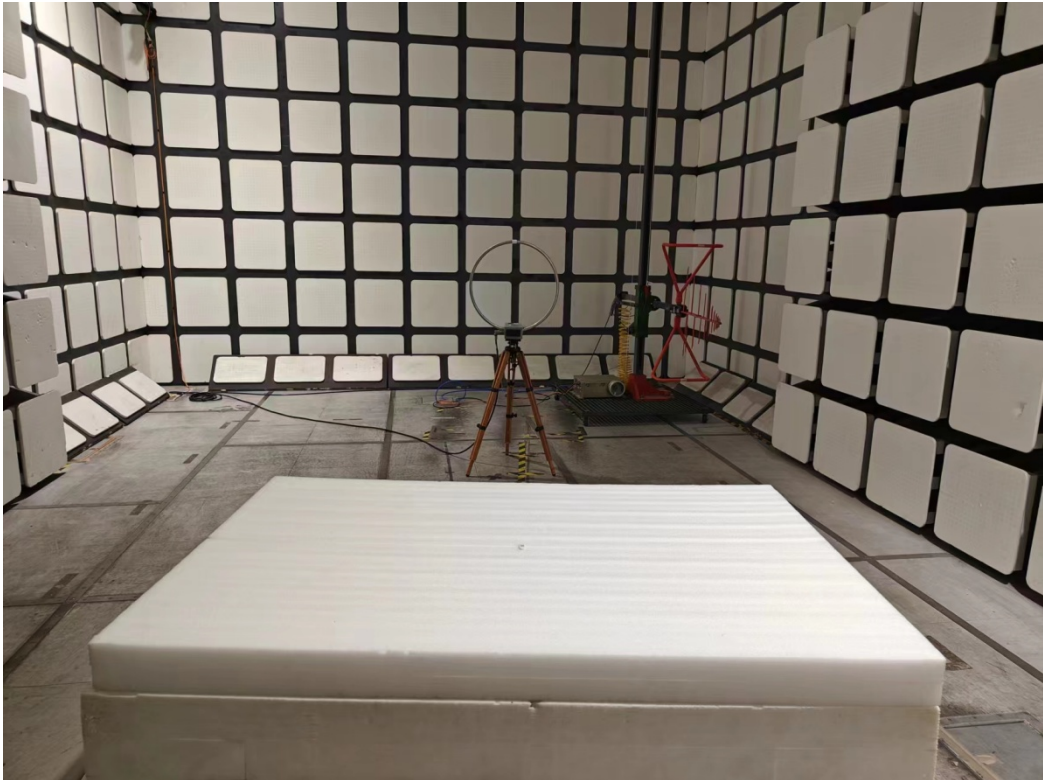
Radiated Emission View (9kHz-30 MHz)
