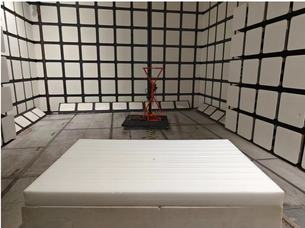
Radiated Emission View (30-1000 MHz)
