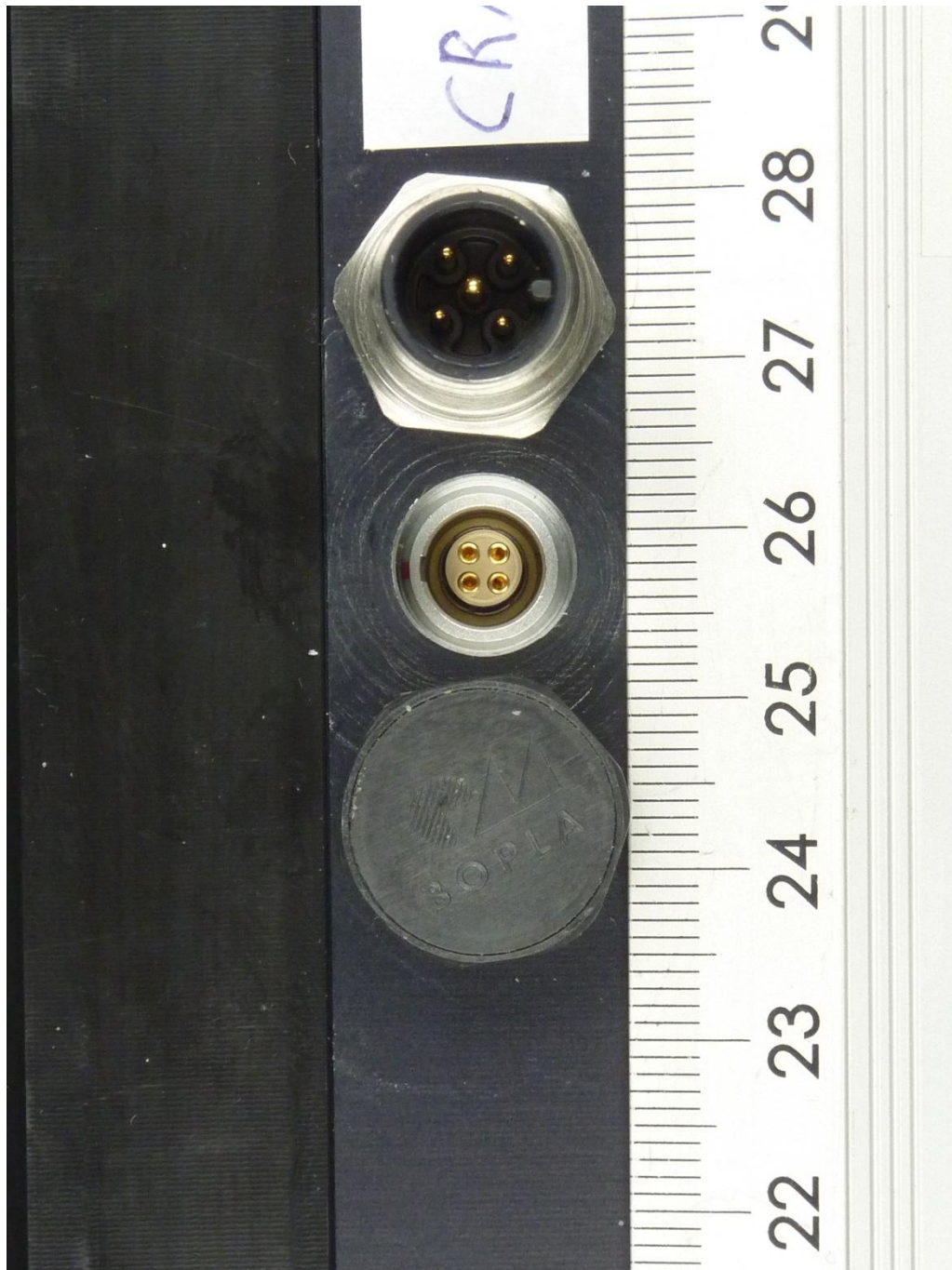
152175_12.JPG: CRAT81, connector view, service interface opened
