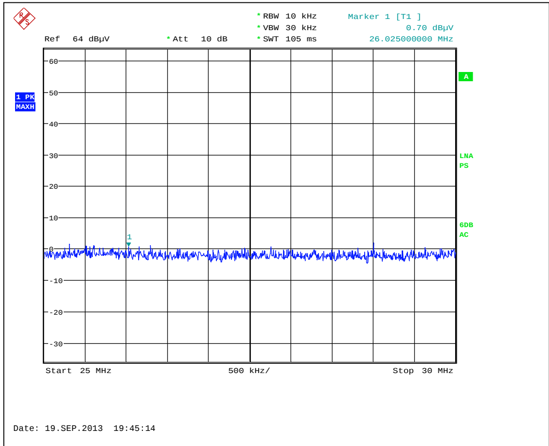
Graph 4.6.2 Horizontal Antenna Polarity
