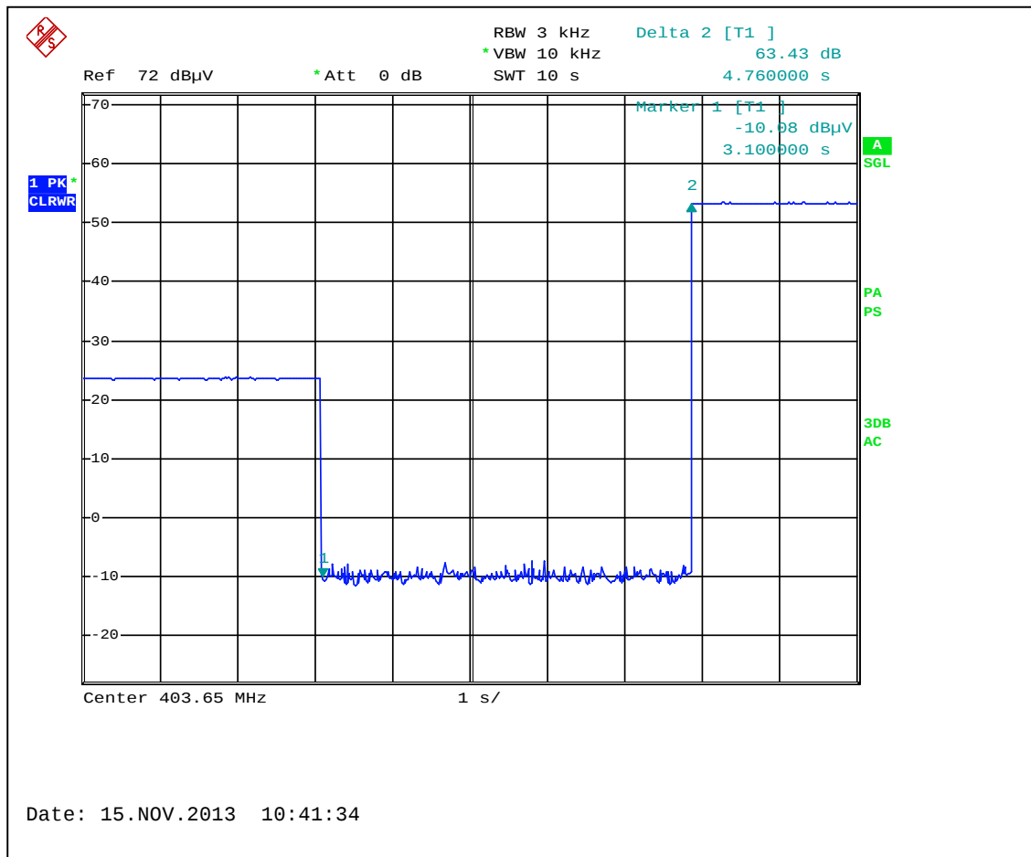
Graph 4.5.4 Scan Cycle Time 3 (4.76sec)
