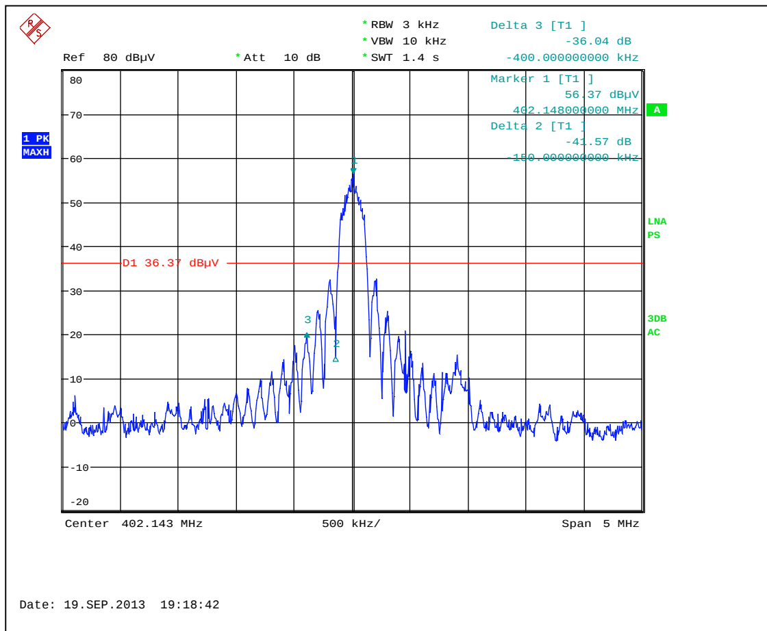
Graph 3.3.4 Lower 250kHz band edge
