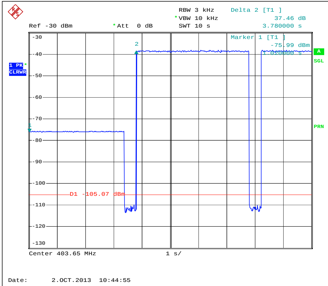
Graph 3.5.3 Scan Cycle Time 2 (3.78sec)
