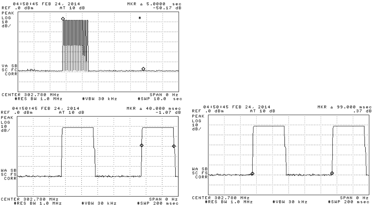
Figure 5: Pulsed Emission Characteristics (Duty Cycle).
