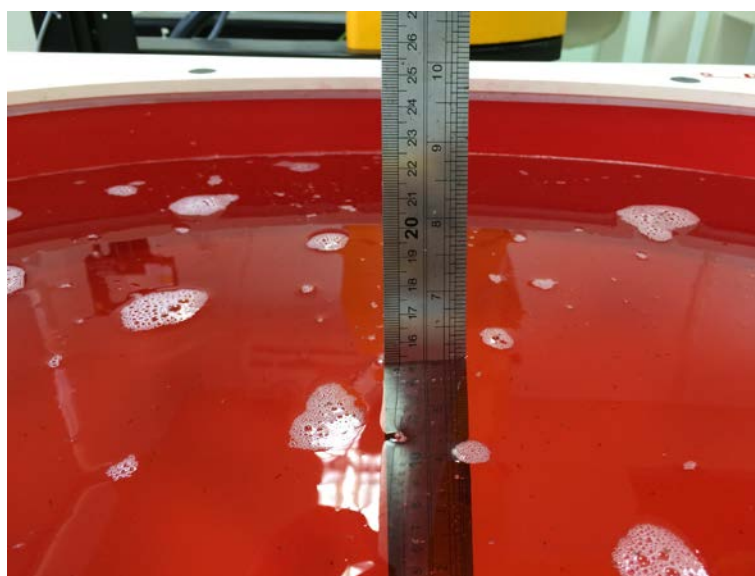
Photograph of the depth in the Body Phantom (450MHz, 15.2cm depth)
