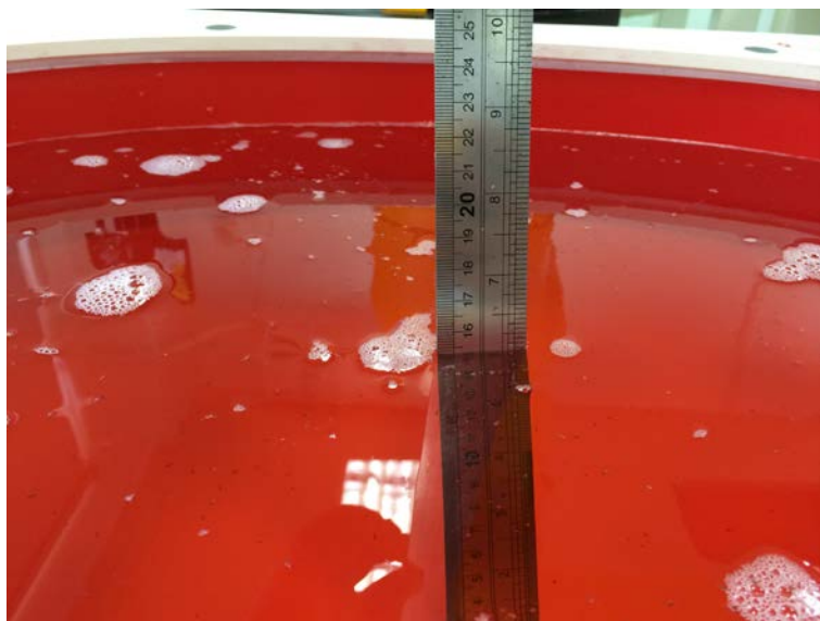
Photograph of the depth in the Head Phantom (450MHz, 15.3cm depth)
