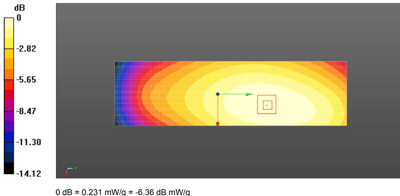
Figure 1: Face held for FM Modulation at 12.5KHz Channel Separation Front towards Phantom 162.10 MHz
