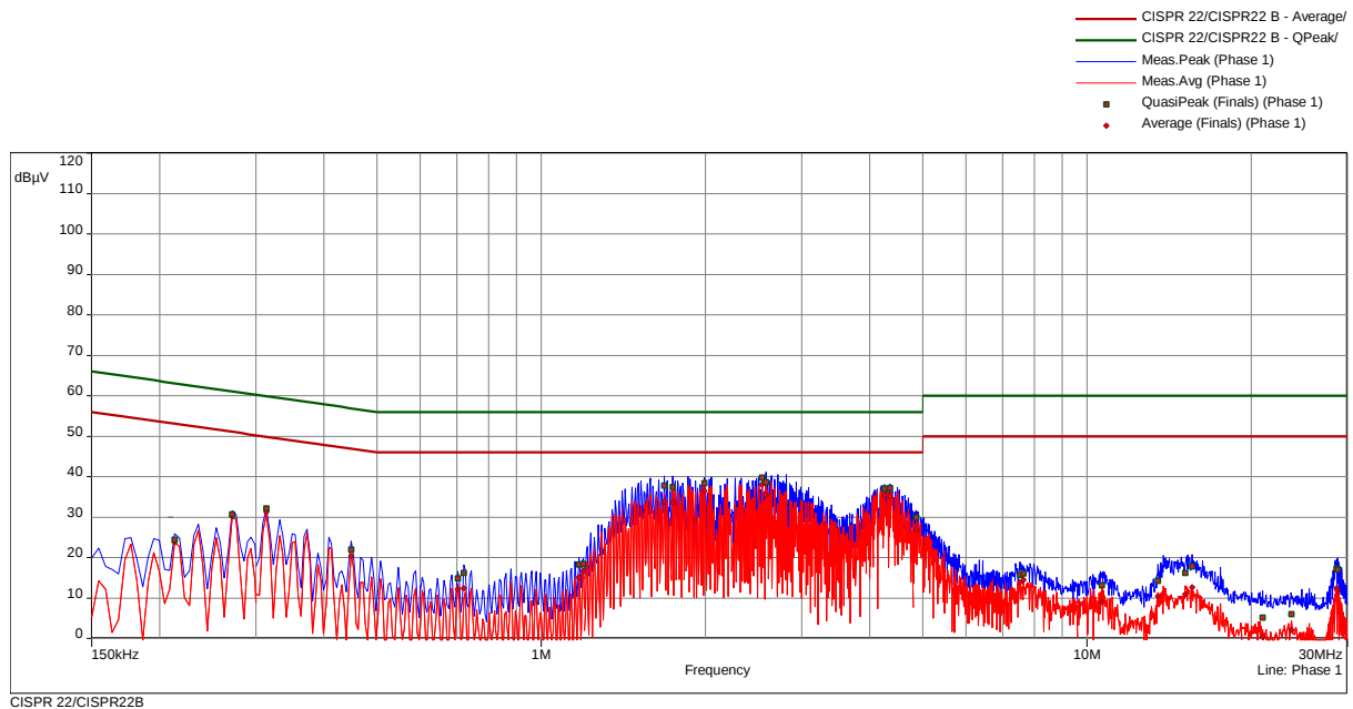
CISPR 22/CISPR22B
