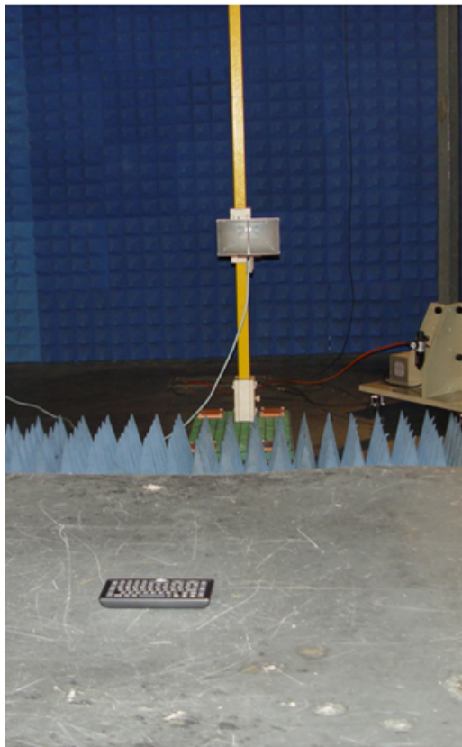
Radiated emissions test > 1GHz
