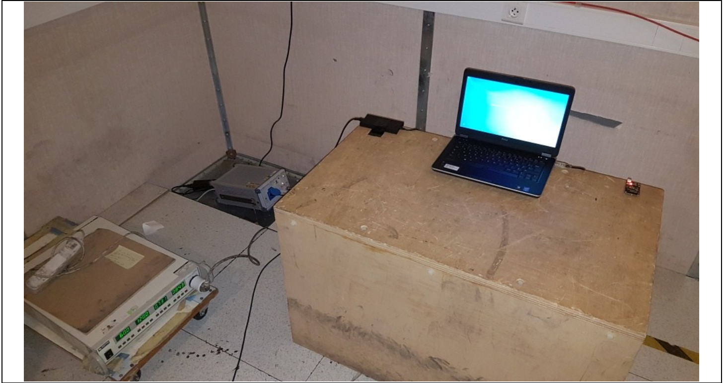
Photograph for AC Power Line Conducted Emissions (Global view)
