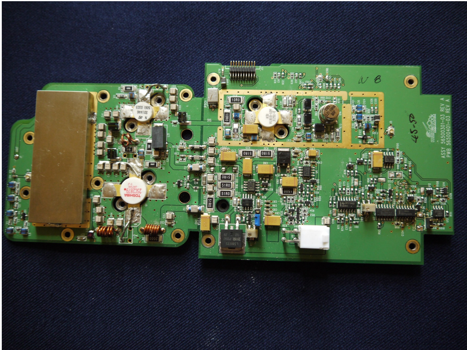
MRC565-430-43 RPA PCB Top with minor shield
