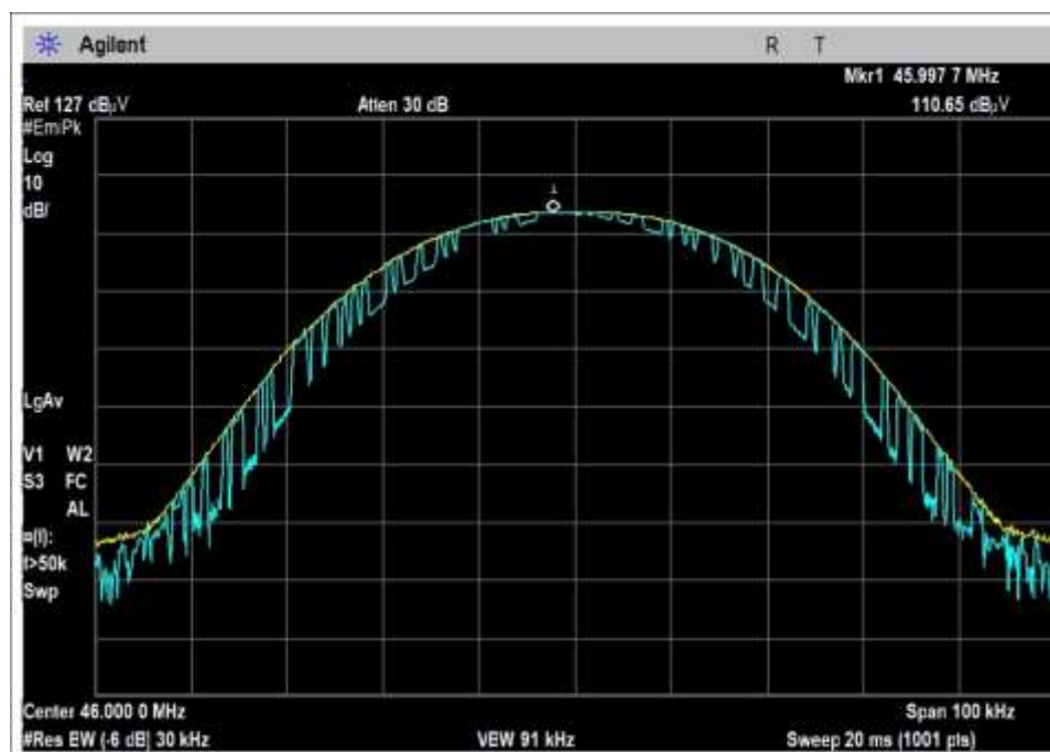
46MHz, 25W
