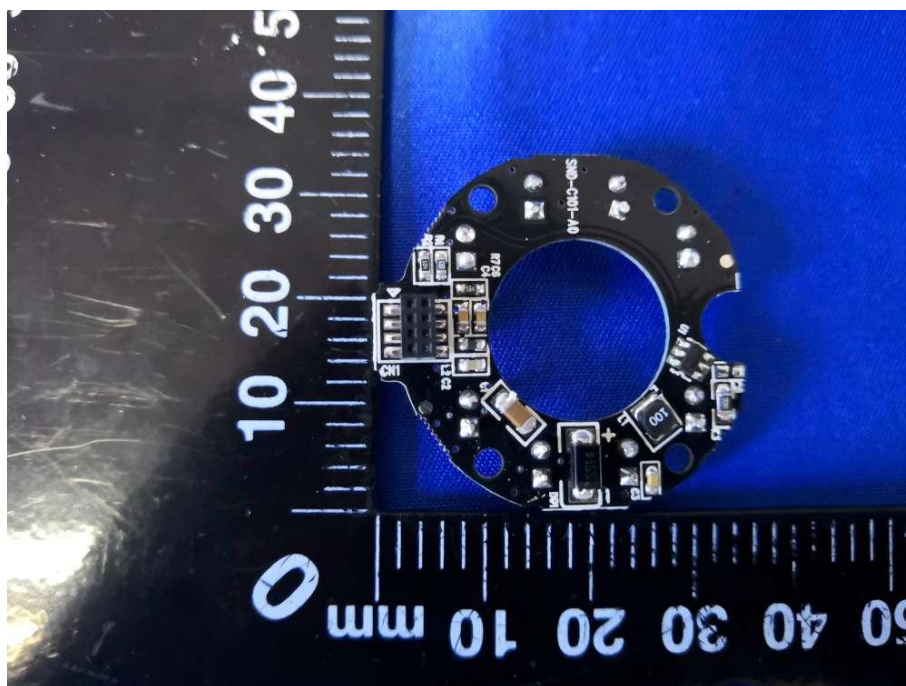
PCB 1 – Front View
