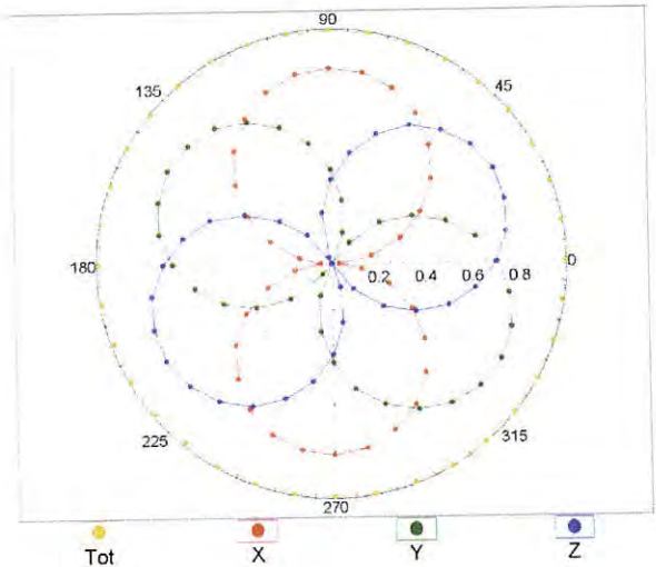
f=600 MHz,TEM
