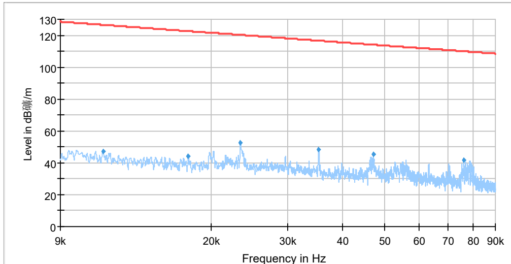
Radiates Emission from 9kHz to 90kHz
