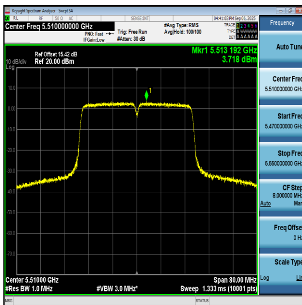
11AC40SISO-Ant2-5510-PASS
