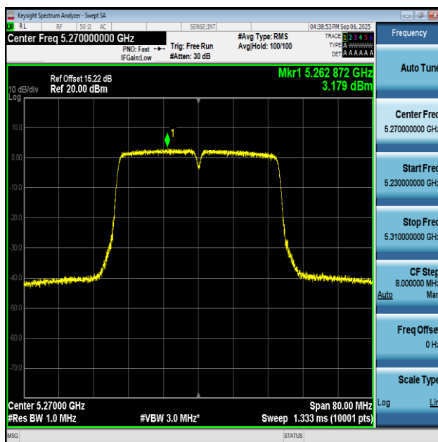
11AC40SISO-Ant2-5270-PASS
