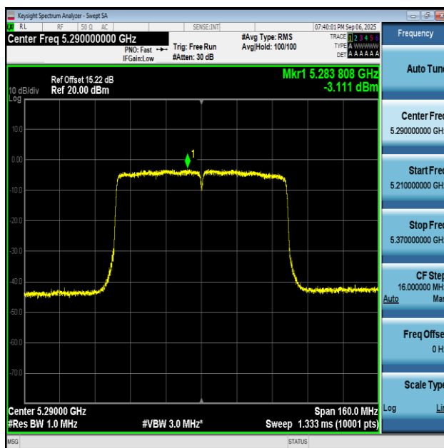
11AC80MIMO-Ant2-5290-PASS
