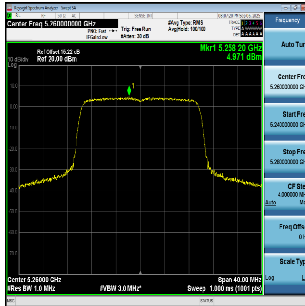
11AX20SISO-Ant1-5260-PASS
