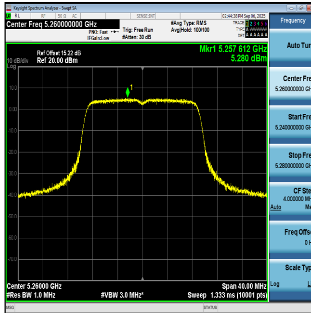
11AC20SISO-Ant1-5260-PASS
