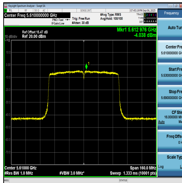
11AC80MIMO-Ant2-5610-PASS
