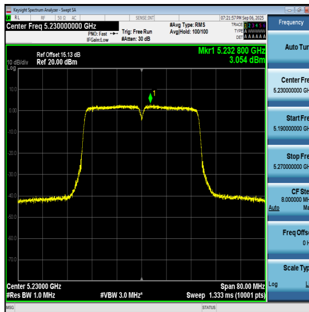
11AC40MIMO-Ant2-5230-PASS
