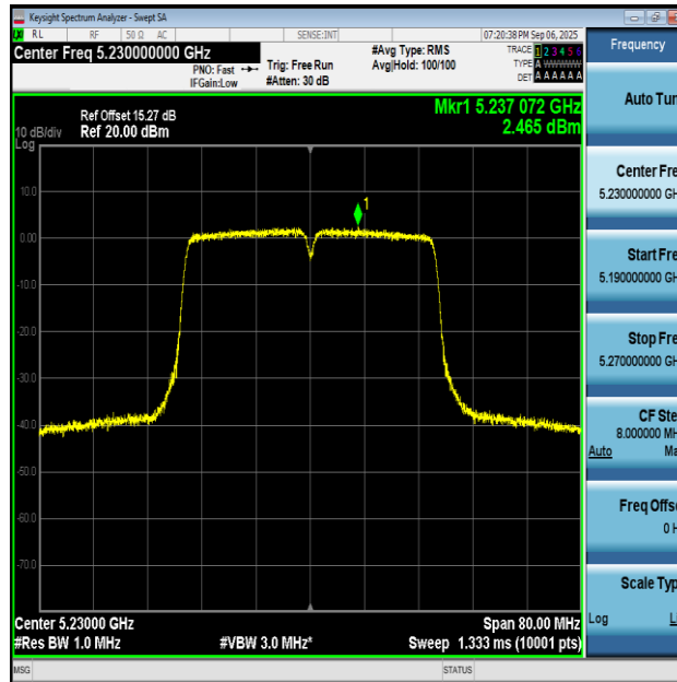
11AC40MIMO-Ant1-5230-PASS
