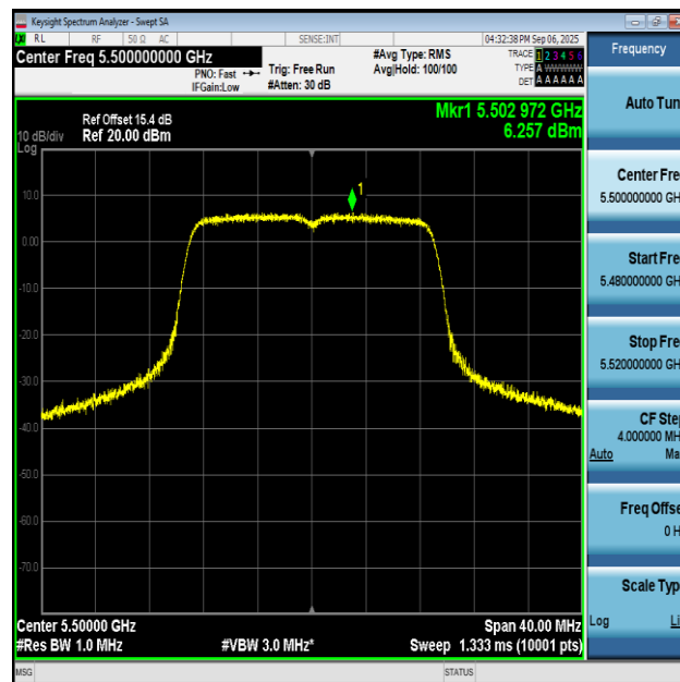
11AC20SISO-Ant2-5500-PASS
