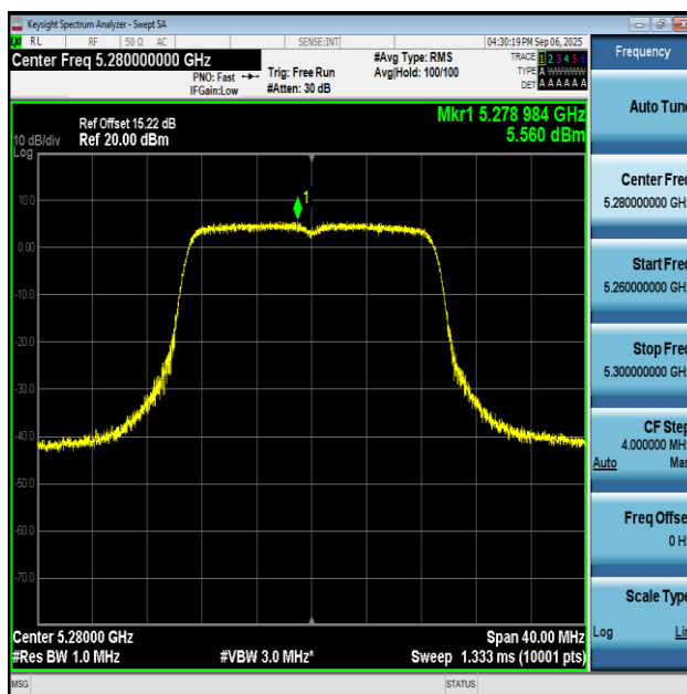
11AC20SISO-Ant2-5280-PASS
