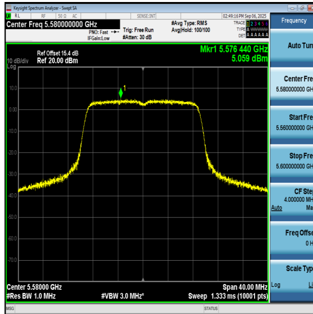
11AC20SISO-Ant1-5580-PASS
