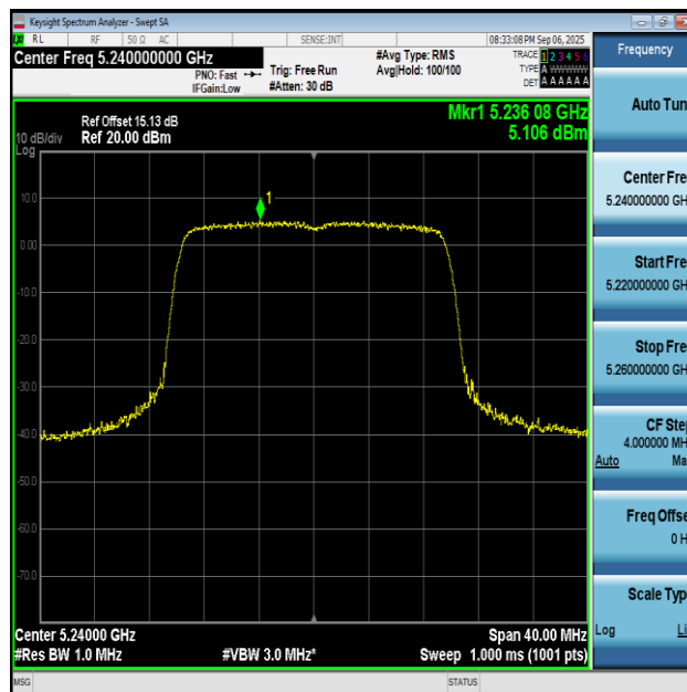
11AX20SISO-Ant2-5240-PASS
