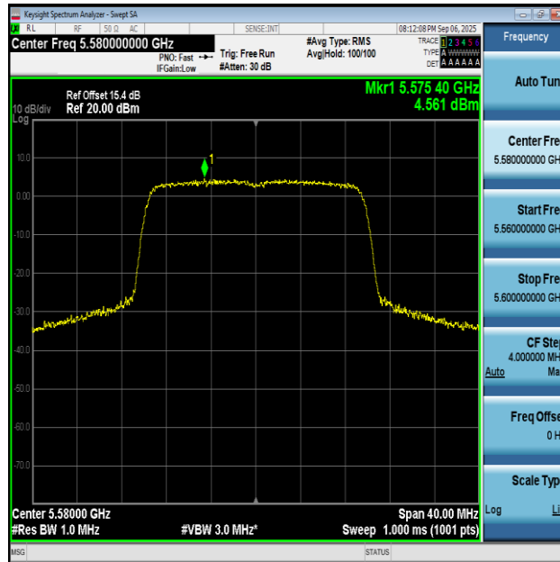
11AX20SISO-Ant1-5580-PASS
