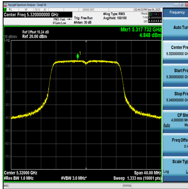
11AC20SISO-Ant1-5320-PASS
