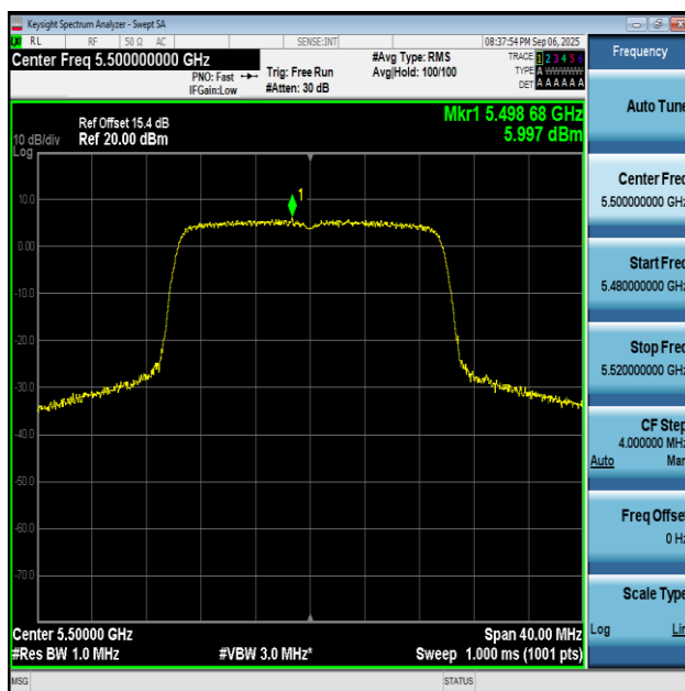
11AX20SISO-Ant2-5500-PASS
