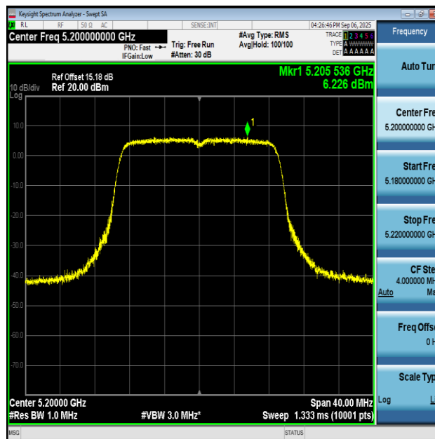
11AC20SISO-Ant2-5200-PASS
