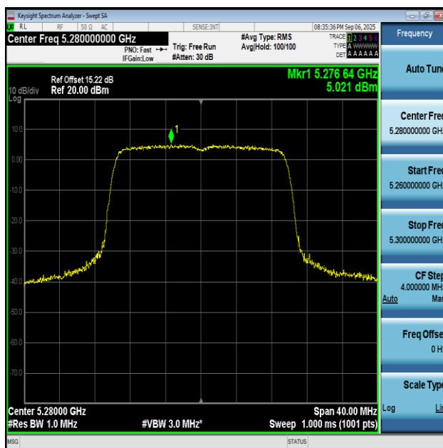
11AX20SISO-Ant2-5280-PASS
