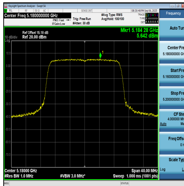
11AX20SISO-Ant2-5180-PASS
