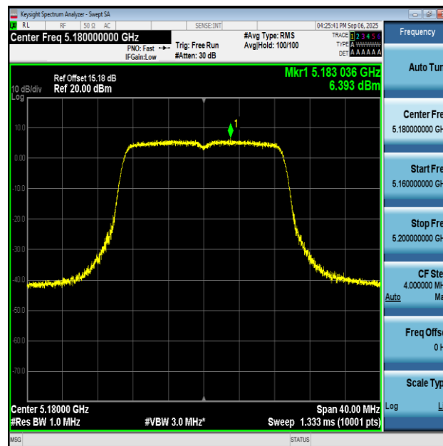
11AC20SISO-Ant2-5180-PASS
