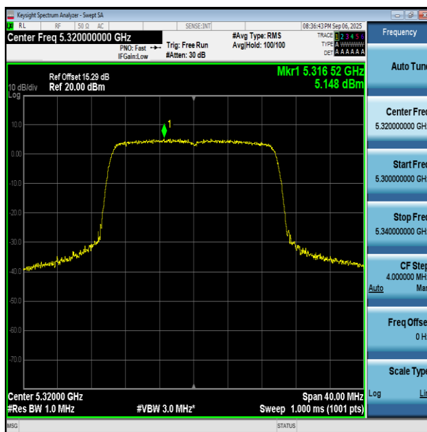
11AX20SISO-Ant2-5320-PASS
