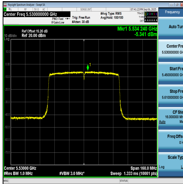
11AC80MIMO-Ant1-5530-PASS
