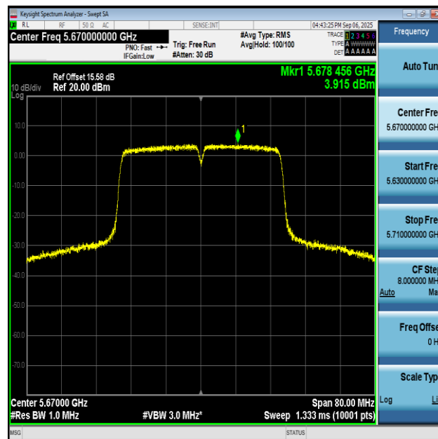
11AC40SISO-Ant2-5670-PASS
