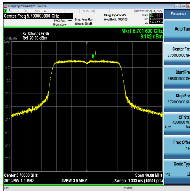
11AC20SISO-Ant2-5700-PASS
