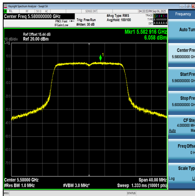
11AC20SISO-Ant2-5580-PASS
