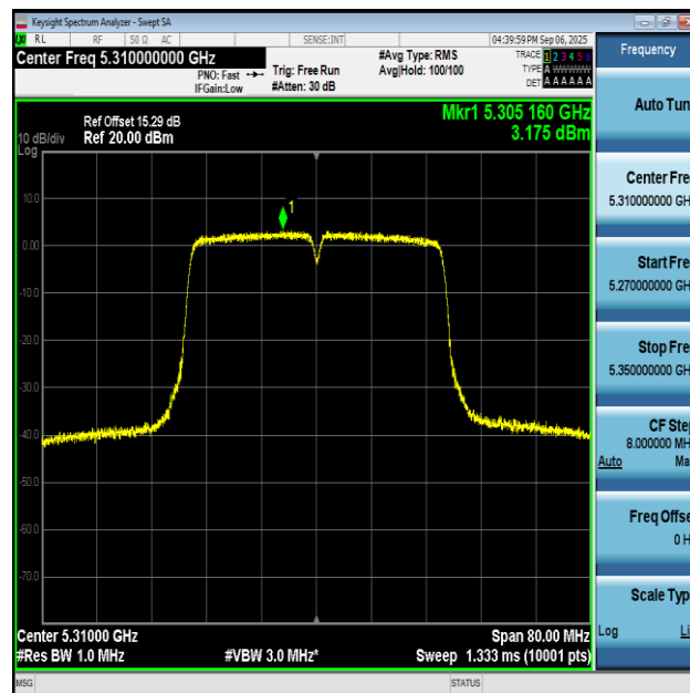
11AC40SISO-Ant2-5310-PASS
