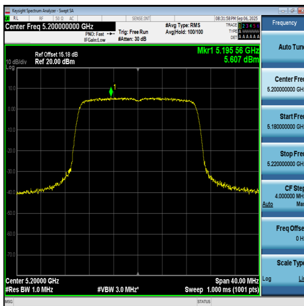
11AX20SISO-Ant2-5200-PASS
