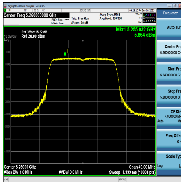
11AC20SISO-Ant2-5260-PASS
