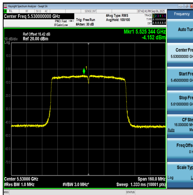
11AC80MIMO-Ant2-5530-PASS
