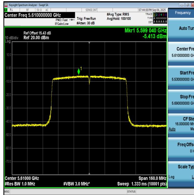
11AC80MIMO-Ant1-5610-PASS
