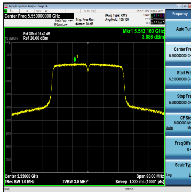
11AC40SISO-Ant2-5550-PASS
