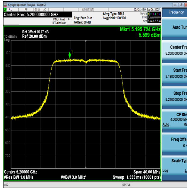
11AC20SISO-Ant1-5200-PASS
