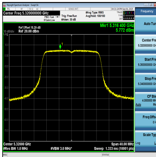
11AC20SISO-Ant2-5320-PASS
