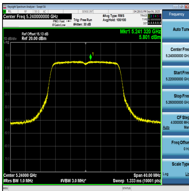
11AC20SISO-Ant2-5240-PASS
