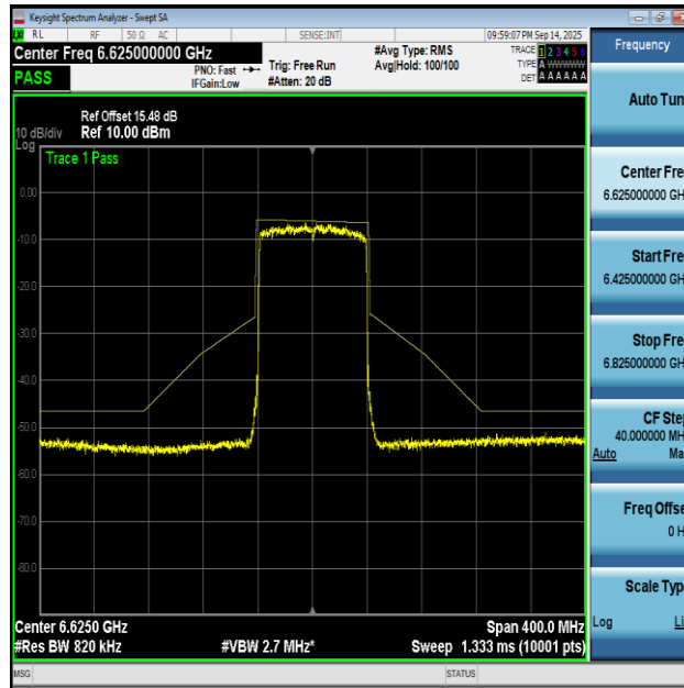
NTNV-11AX80MIMO-Ant1-6625-PASS
