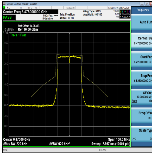
NTNV-11AX20MIMO-Ant1-6475-PASS
