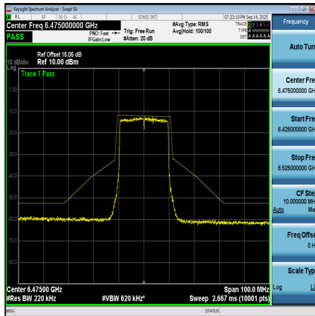
NTNV-11AX20MIMO-Ant2-6475-PASS
