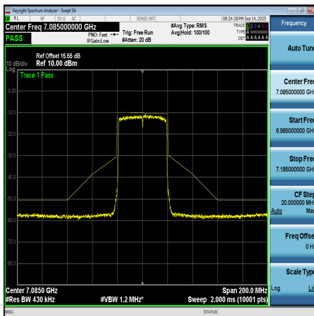
NTNV-11AX40MIMO-Ant1-7085-PASS
