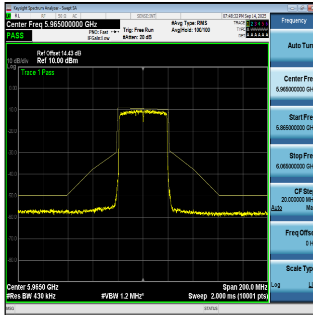
NTNV-11AX40MIMO-Ant1-5965-PASS
