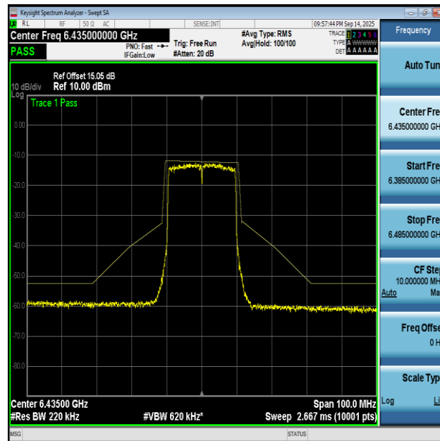
NTNV-11AX20MIMO-Ant2-6435-PASS
