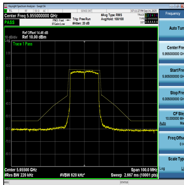
NTNV-11AX20MIMO-Ant2-5955-PASS
