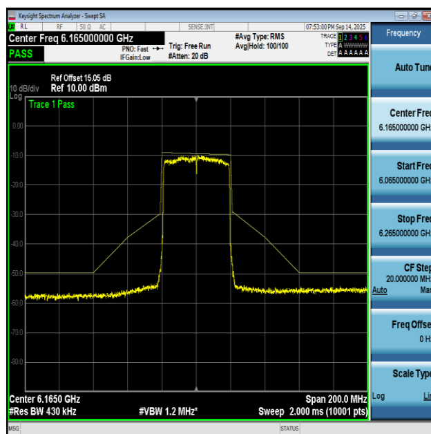
NTNV-11AX40MIMO-Ant2-6165-PASS
