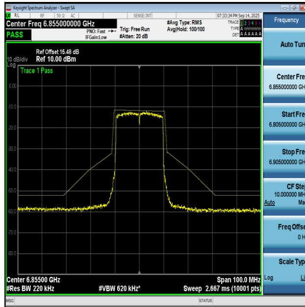
NTNV-11AX20MIMO-Ant1-6855-PASS
