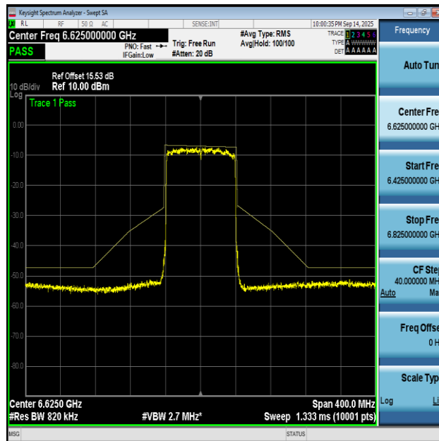
NTNV-11AX80MIMO-Ant2-6625-PASS
