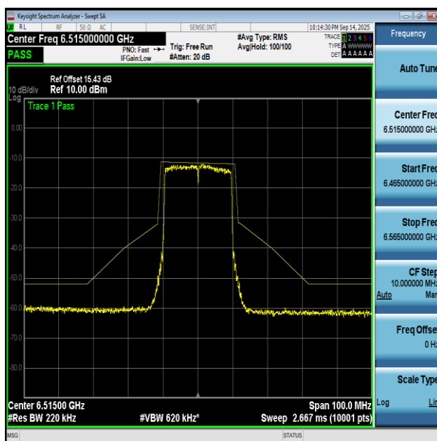
NTNV-11AX20MIMO-Ant2-6515-PASS
