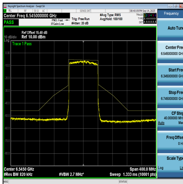
NTNV-11AX80MIMO-Ant1-6545-PASS
