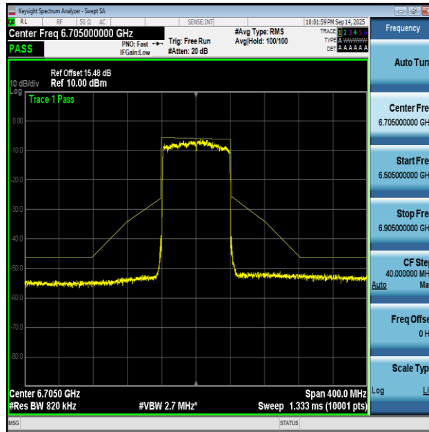
NTNV-11AX80MIMO-Ant1-6705-PASS
