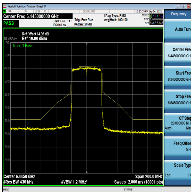
NTNV-11AX40MIMO-Ant1-6445-PASS
