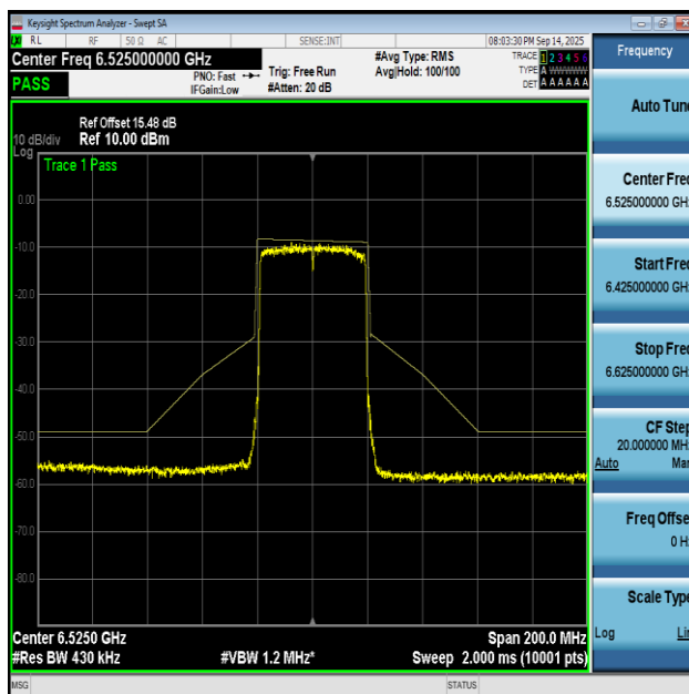
NTNV-11AX40MIMO-Ant1-6525-PASS
