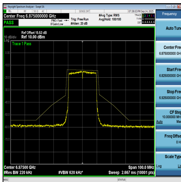
NTNV-11AX20MIMO-Ant2-6875-PASS
