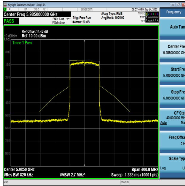
NTNV-11AX80MIMO-Ant1-5985-PASS
