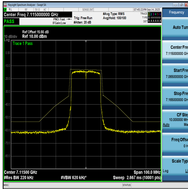
NTNV-11AX20MIMO-Ant1-7115-PASS
