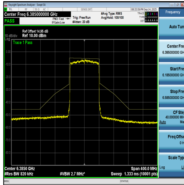
NTNV-11AX80MIMO-Ant1-6385-PASS
