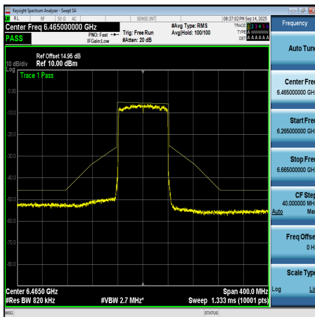
NTNV-11AX80MIMO-Ant1-6465-PASS
