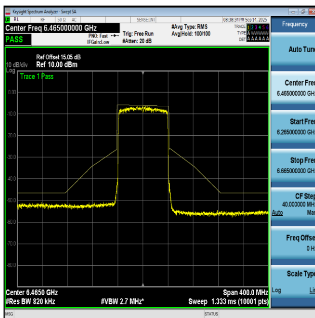
NTNV-11AX80MIMO-Ant2-6465-PASS
