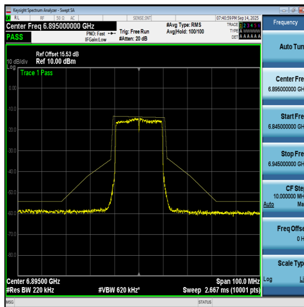
NTNV-11AX20MIMO-Ant2-6895-PASS
