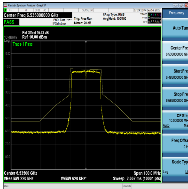
NTNV-11AX20MIMO-Ant2-6535-PASS
