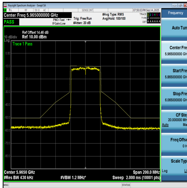
NTNV-11AX40MIMO-Ant2-5965-PASS
