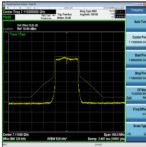
NTNV-11AX20MIMO-Ant2-7115-PASS
