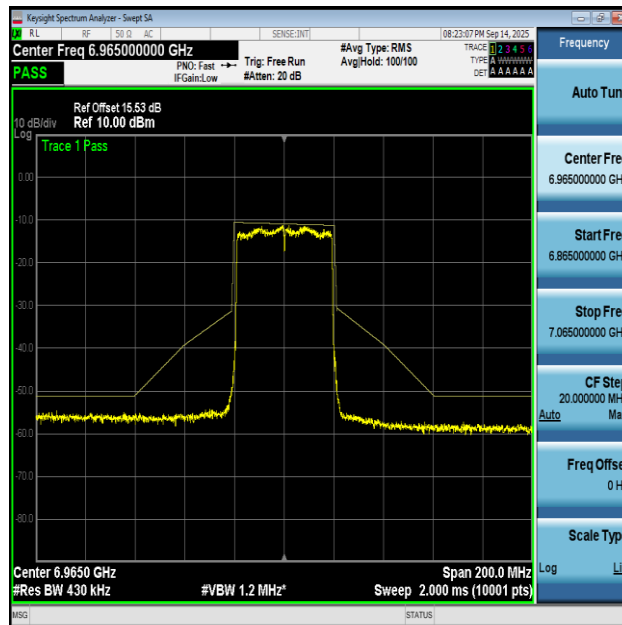
NTNV-11AX40MIMO-Ant2-6965-PASS
