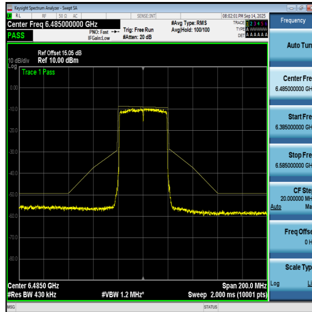
NTNV-11AX40MIMO-Ant2-6485-PASS
