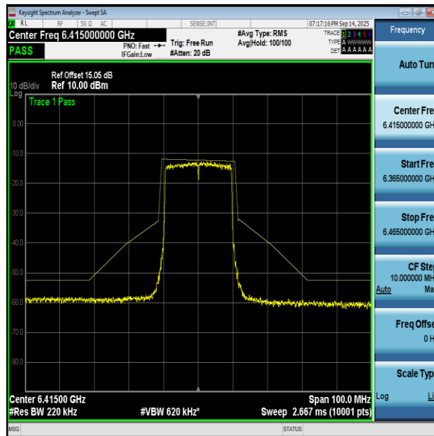
NTNV-11AX20MIMO-Ant2-6415-PASS
