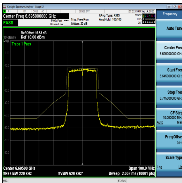
NTNV-11AX20MIMO-Ant2-6695-PASS
