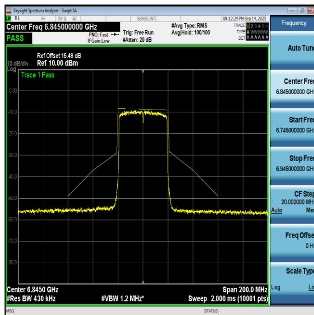
NTNV-11AX40MIMO-Ant1-6845-PASS
