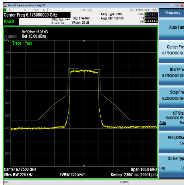
NTNV-11AX20MIMO-Ant2-6175-PASS
