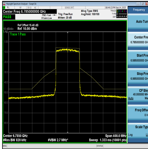
NTNV-11AX80MIMO-Ant1-6785-PASS
