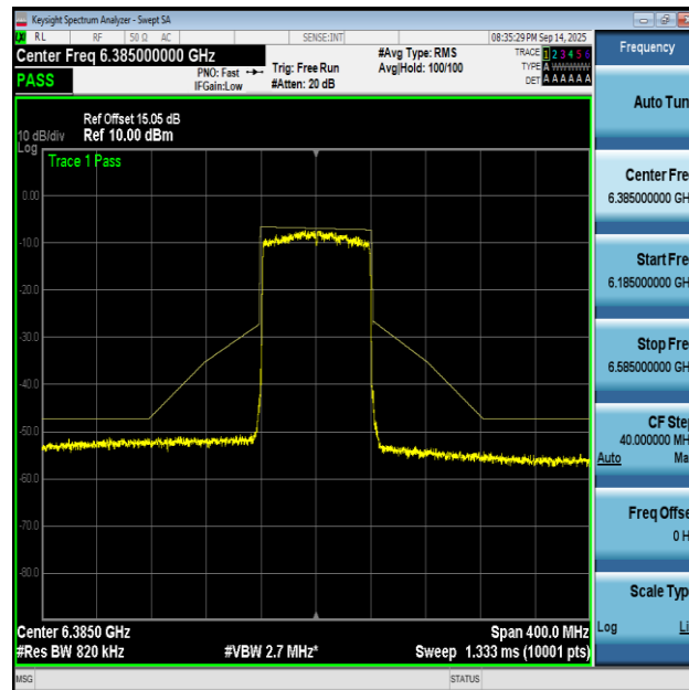
NTNV-11AX80MIMO-Ant2-6385-PASS
