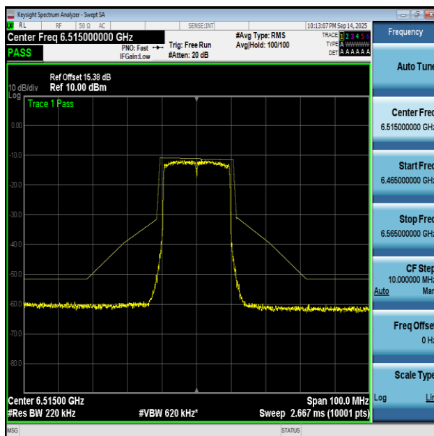
NTNV-11AX20MIMO-Ant1-6515-PASS
