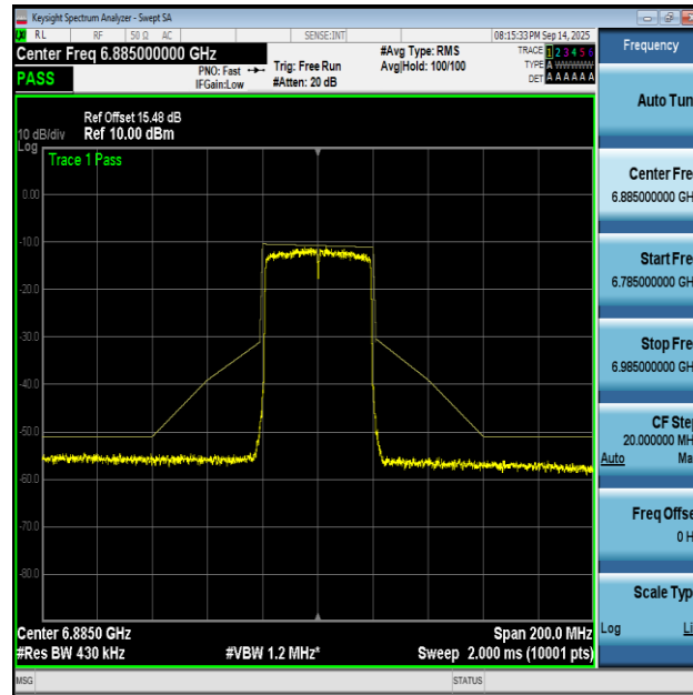
NTNV-11AX40MIMO-Ant1-6885-PASS
