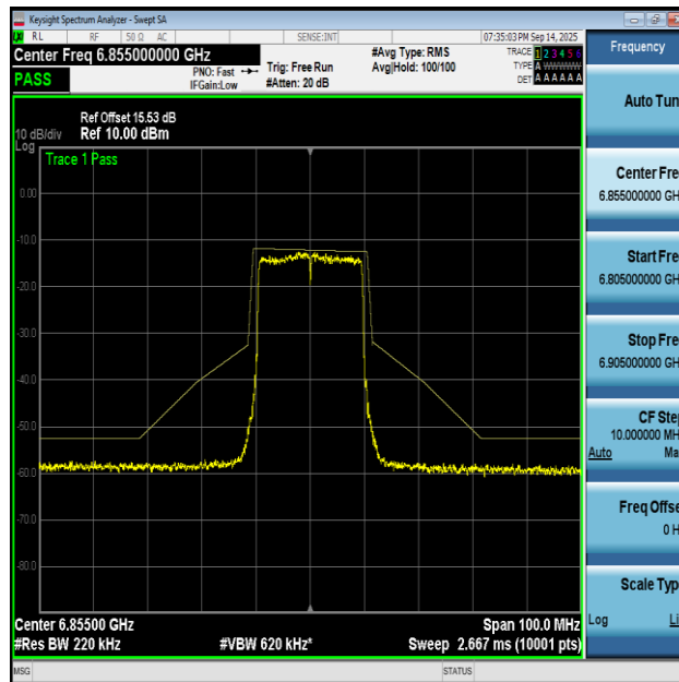
NTNV-11AX20MIMO-Ant2-6855-PASS
