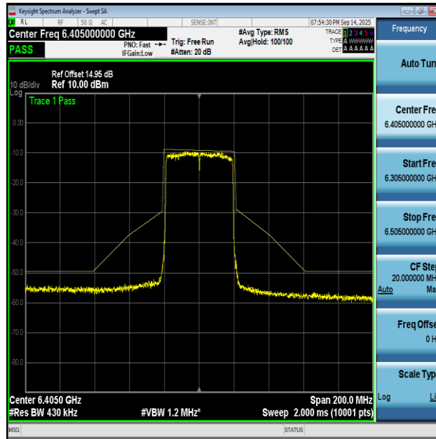
NTNV-11AX40MIMO-Ant1-6405-PASS
