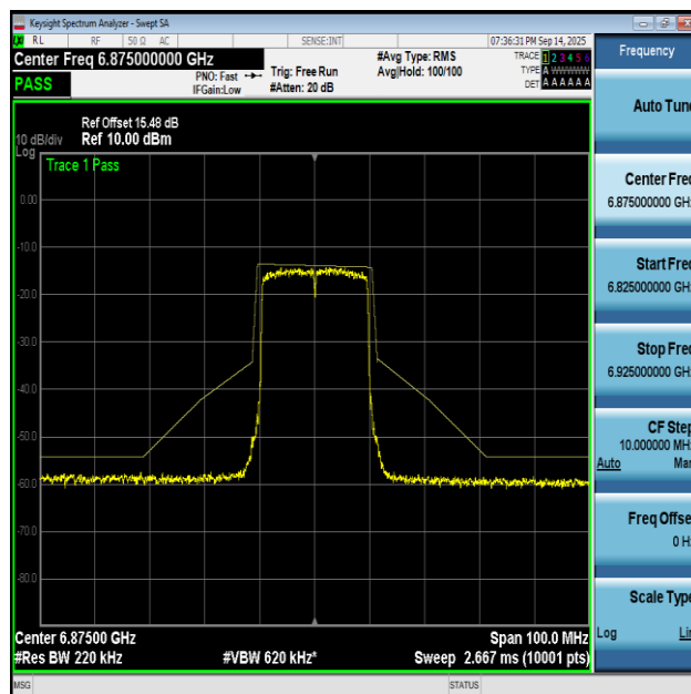
NTNV-11AX20MIMO-Ant1-6875-PASS
