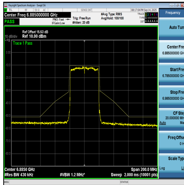
NTNV-11AX40MIMO-Ant2-6885-PASS
