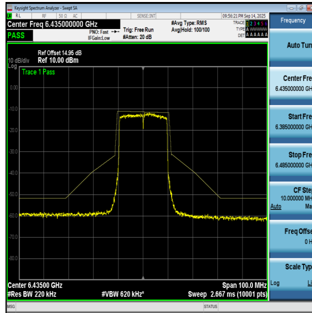
NTNV-11AX20MIMO-Ant1-6435-PASS
