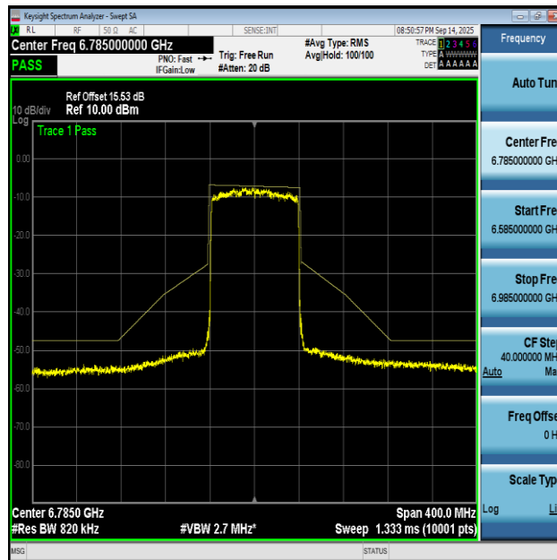
NTNV-11AX80MIMO-Ant2-6785-PASS
