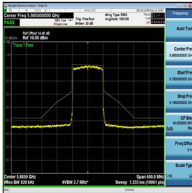
NTNV-11AX80MIMO-Ant2-5985-PASS
