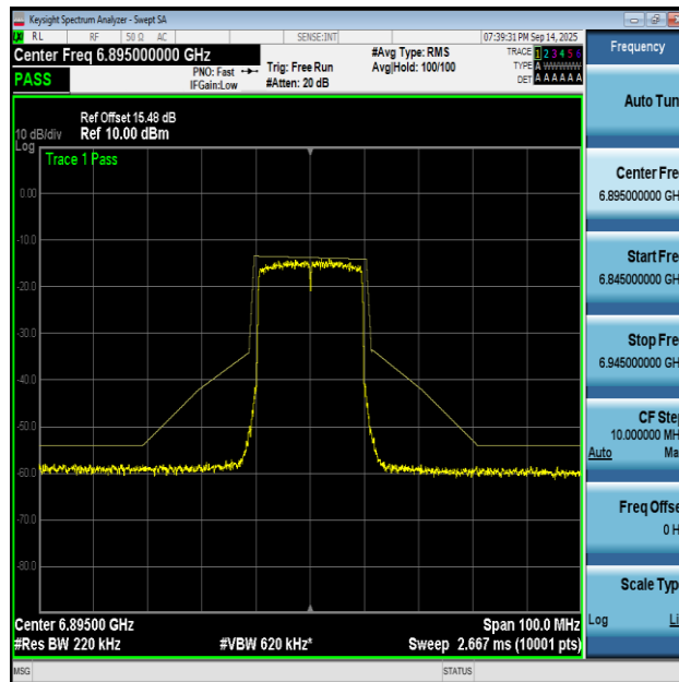
NTNV-11AX20MIMO-Ant1-6895-PASS
