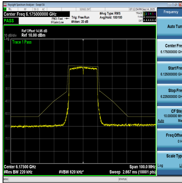
NTNV-11AX20MIMO-Ant1-6175-PASS
