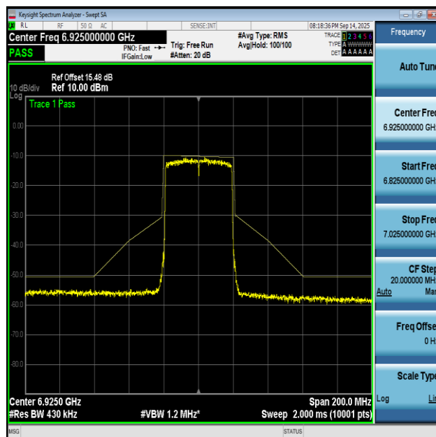
NTNV-11AX40MIMO-Ant1-6925-PASS
