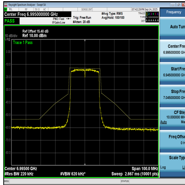
NTNV-11AX20MIMO-Ant1-6995-PASS
