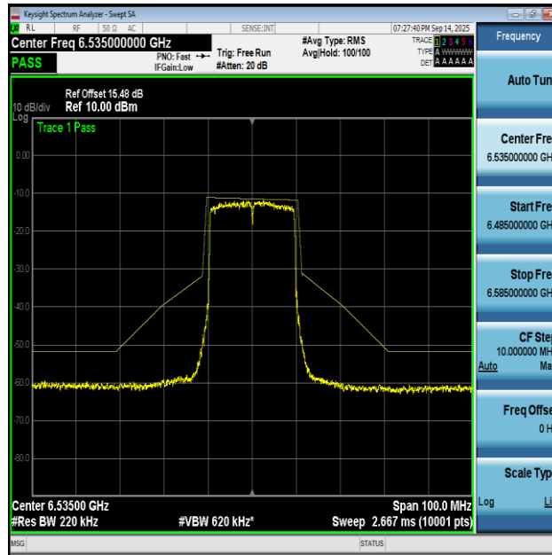
NTNV-11AX20MIMO-Ant1-6535-PASS
