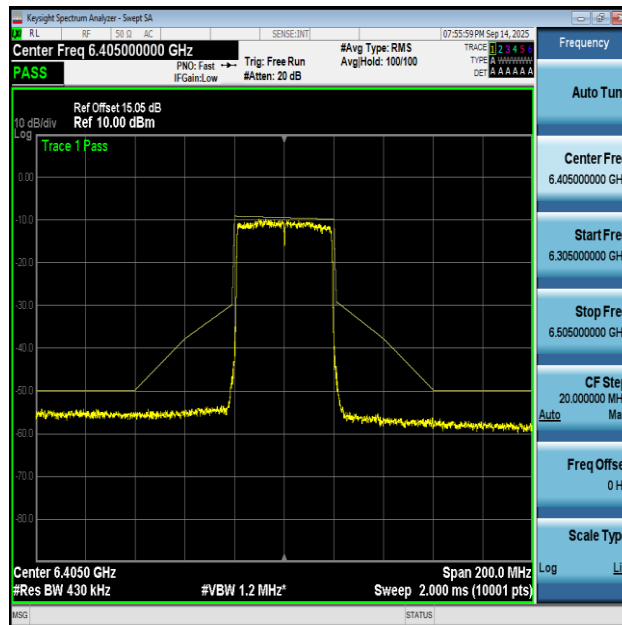
NTNV-11AX40MIMO-Ant2-6405-PASS
