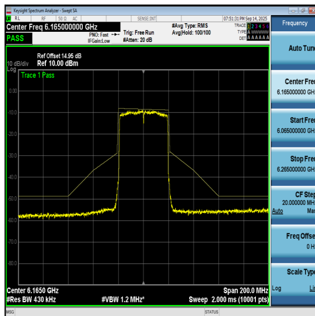
NTNV-11AX40MIMO-Ant1-6165-PASS
