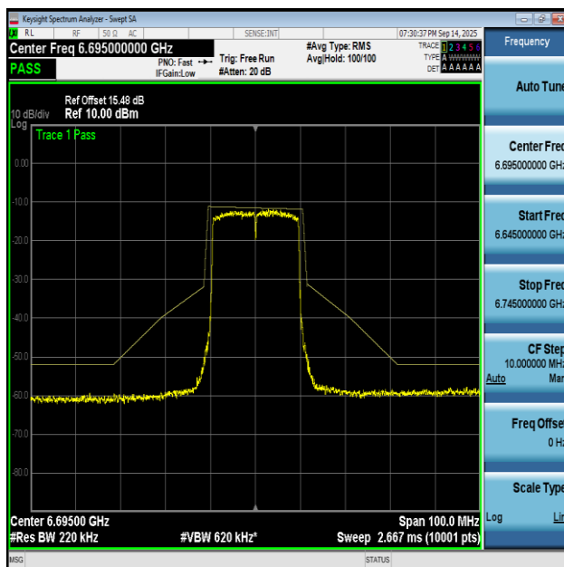
NTNV-11AX20MIMO-Ant1-6695-PASS
