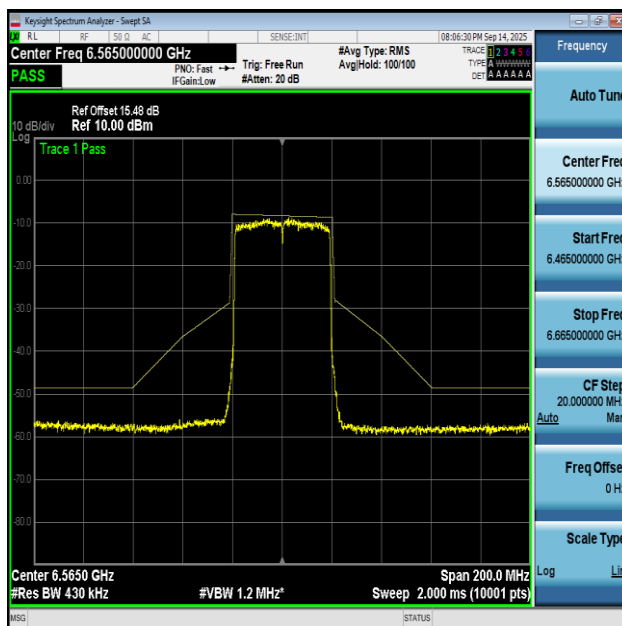
NTNV-11AX40MIMO-Ant1-6565-PASS
