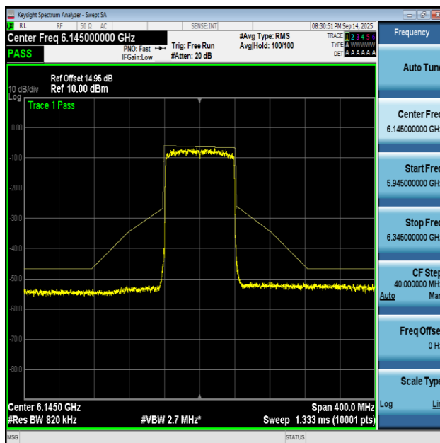
NTNV-11AX80MIMO-Ant1-6145-PASS
