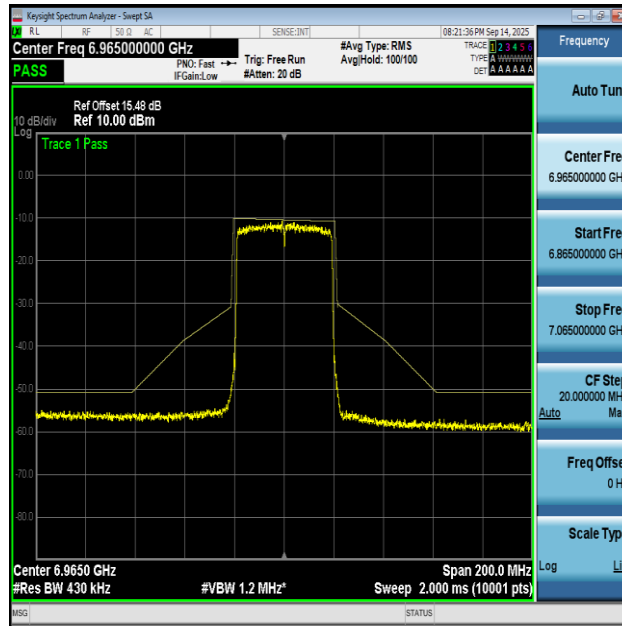
NTNV-11AX40MIMO-Ant1-6965-PASS
