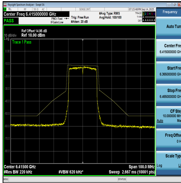
NTNV-11AX20MIMO-Ant1-6415-PASS
