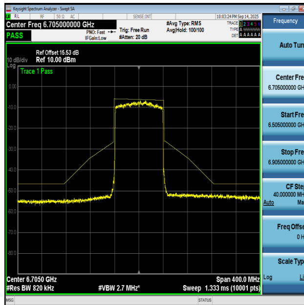
NTNV-11AX80MIMO-Ant2-6705-PASS
