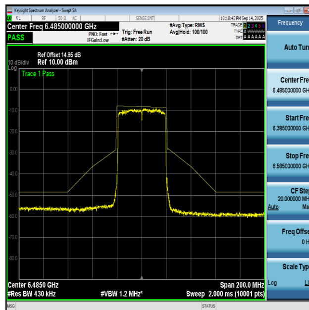
NTNV-11AX40MIMO-Ant1-6485-PASS
