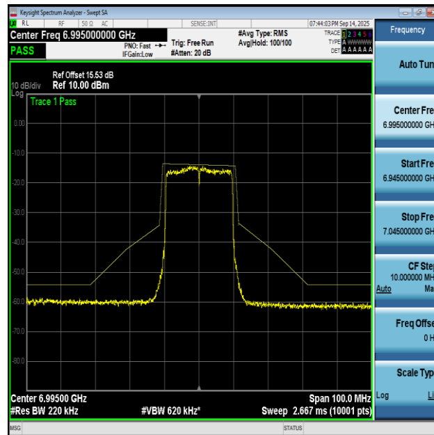
NTNV-11AX20MIMO-Ant2-6995-PASS
