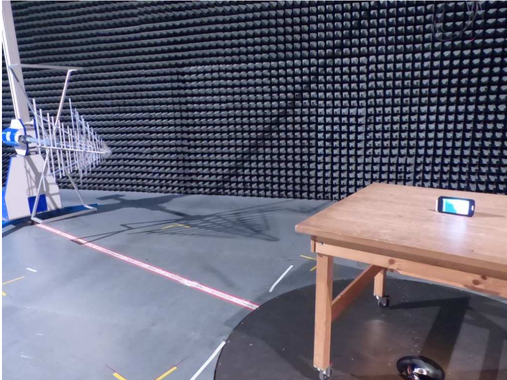
Photo 3: Test setup for radiated measurements (AC Port (power line), EUT supplied by battery, unintentional radiator §15)
