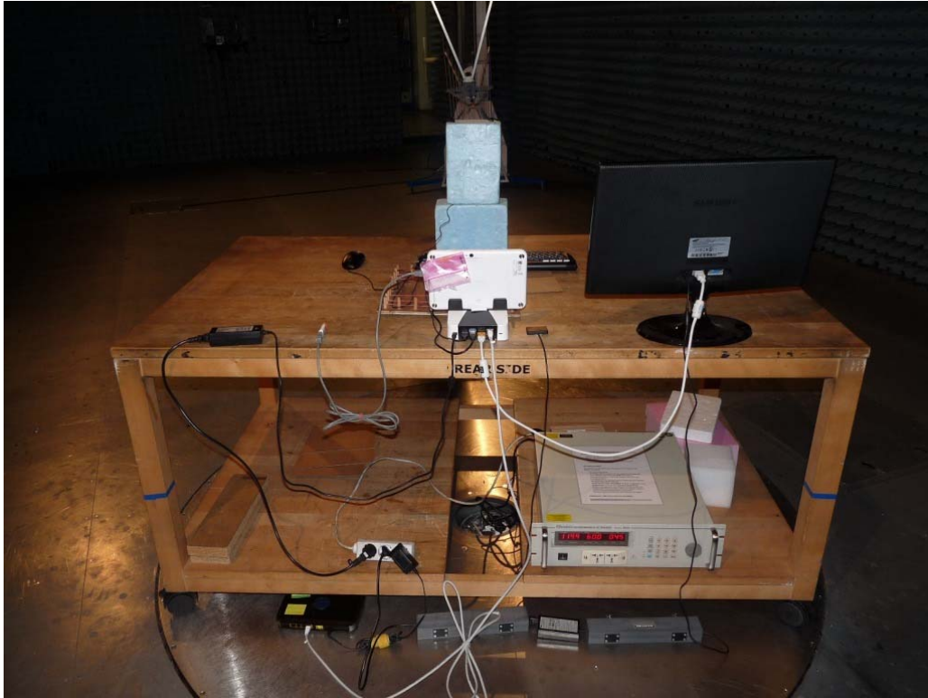
Photo 4: Test setup for radiated measurements (computer peripheral setup, unintentional radiator §15)
