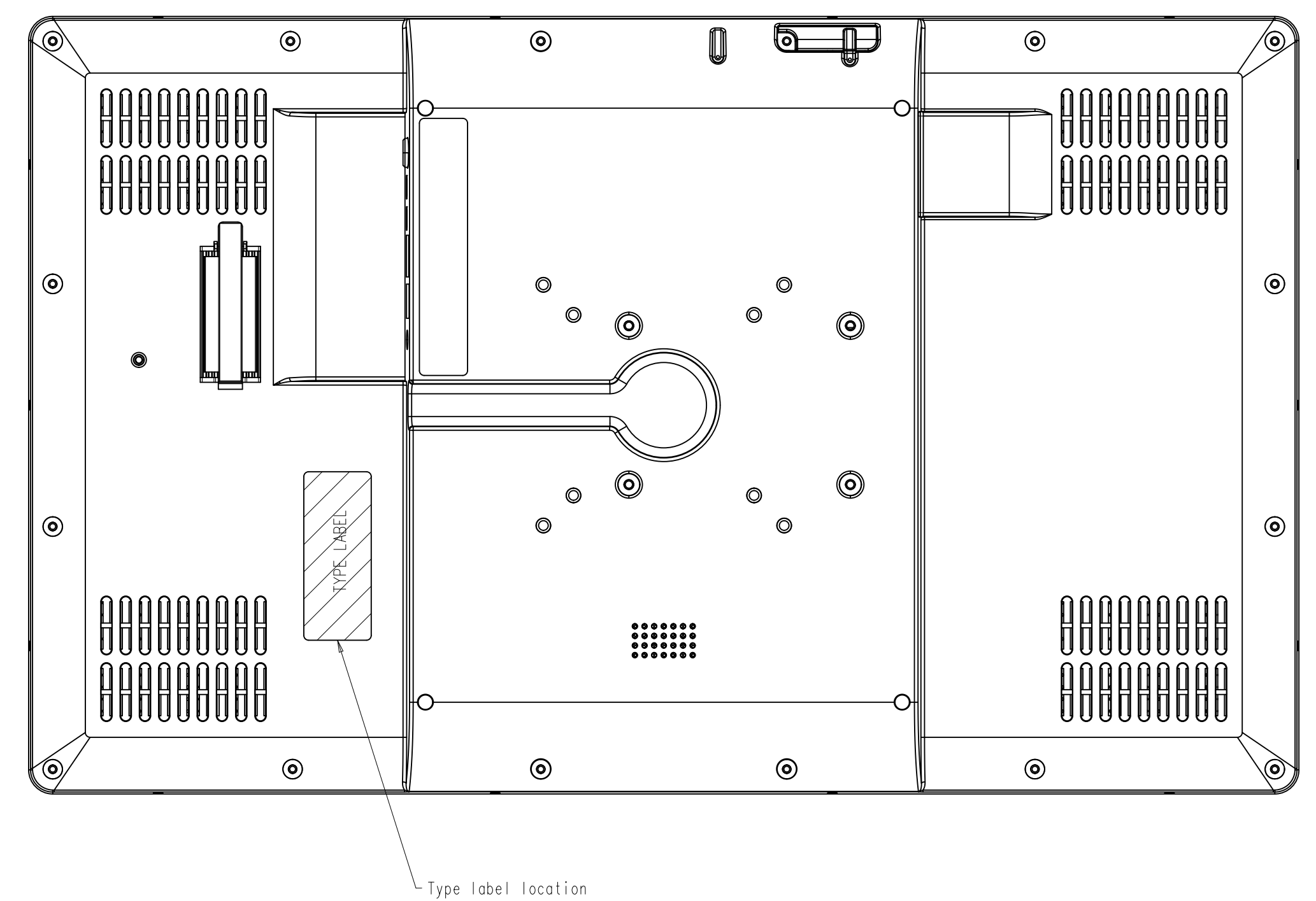
BACK VIEW
