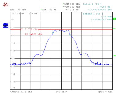
CH19 6 dB Bandwidth
