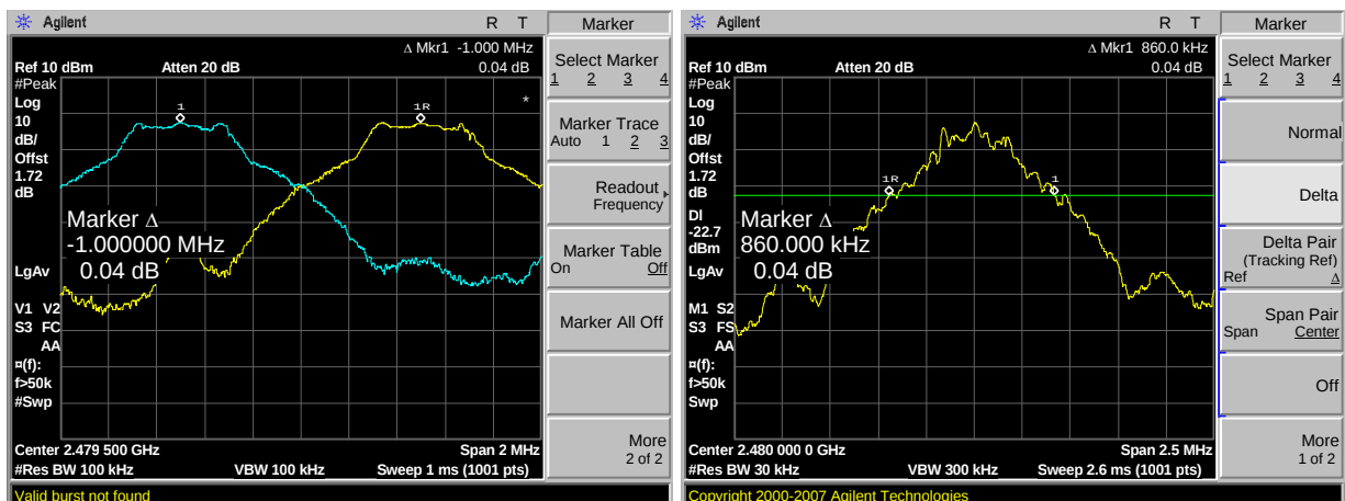
2480 MHz DH3 Frequency Separation / 20 dB Bandwidth
