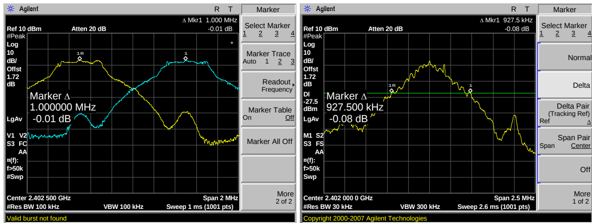
2402 MHz DH5 Frequency Separation / 20 dB Bandwidth
