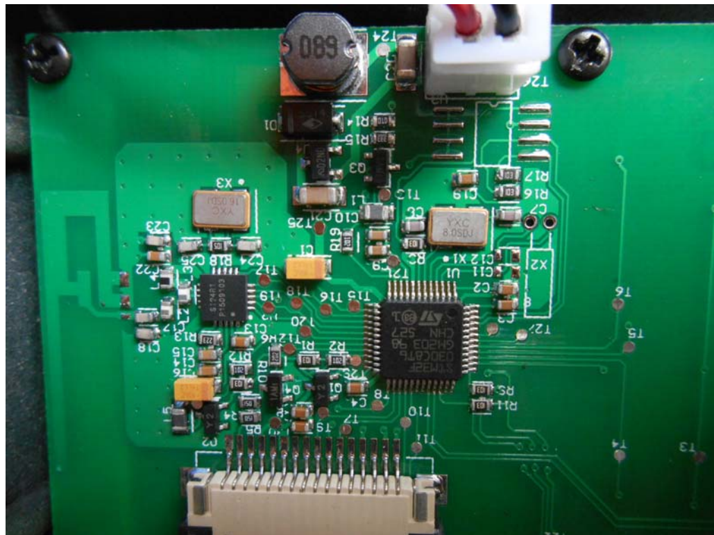
FIGURE 6 ELECTRONIC GAME CALLER (M/N: GS2) CHIP AND CRYSTAL ON KEYBOARD
