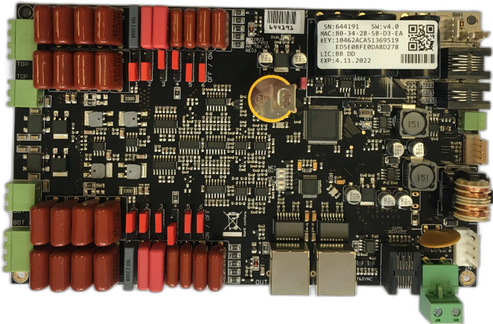
AM TRX board, TOP
