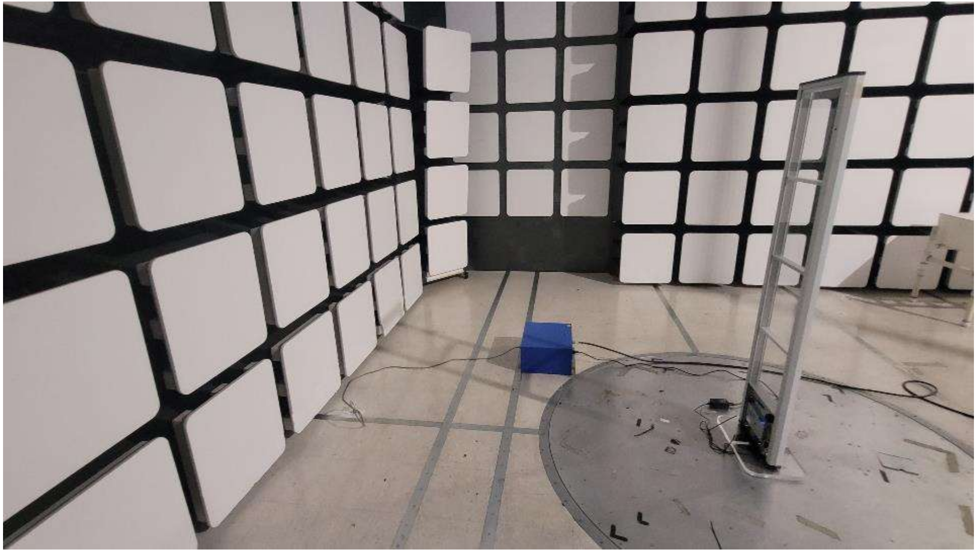
CR - Lab D - 8.2 MHz System - 65 Watt
