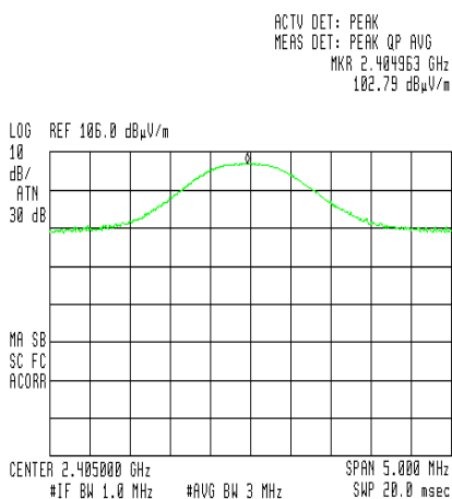
Figure 12. Field Strength of Fundamental. Antenna Polarization: HORIZONTAL Channel: Low
