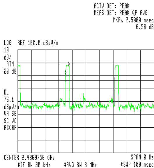
Figure 20. Transmission Burst Duration = 2.5 msec
