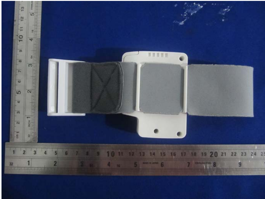
EUT—Bottom View
