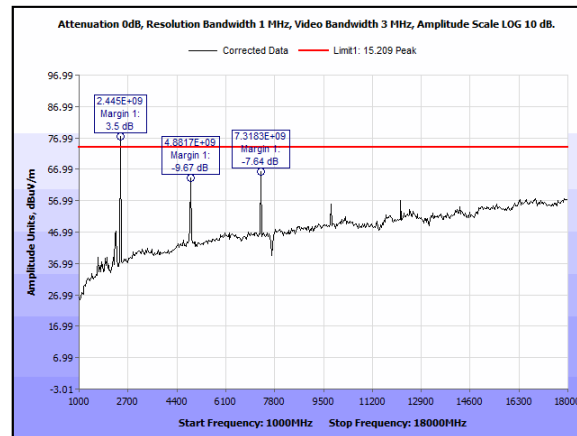
Plot 23. Radiated Emissions, Peak, 1 – 18 GHz, Mid Channel
