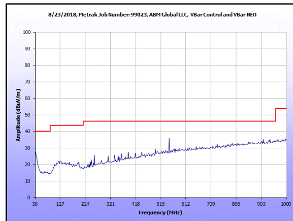
Plot 25. Radiated Emissions, 15.209, 30 MHz - 1 GHz, prescan, Low
