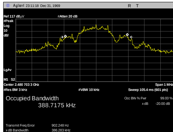
Plot 1. 20 dB Occupied Bandwidth, High Channel, final
