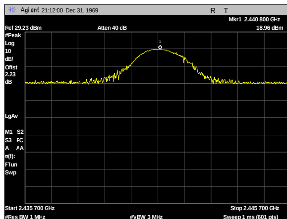
Plot 16. Peak Power Output, 18.96dBm, Mid
