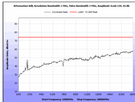
Plot 24. Radiated Emissions, Peak, 1 – 18 GHz, Low Channel
