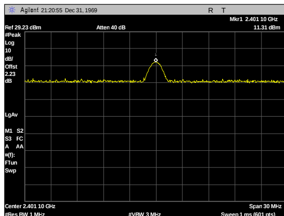
Plot 15. Peak Power Output, 11.31dBm, Low
