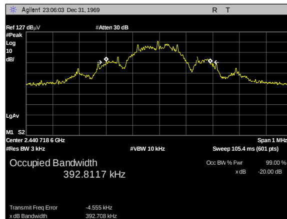
Plot 3. 20 dB Occupied Bandwidth, Mid Channel
