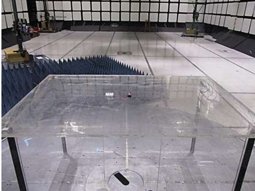
Photograph 5. Radiated Emissions, (1 GHz – 18 GHz), Rear View
