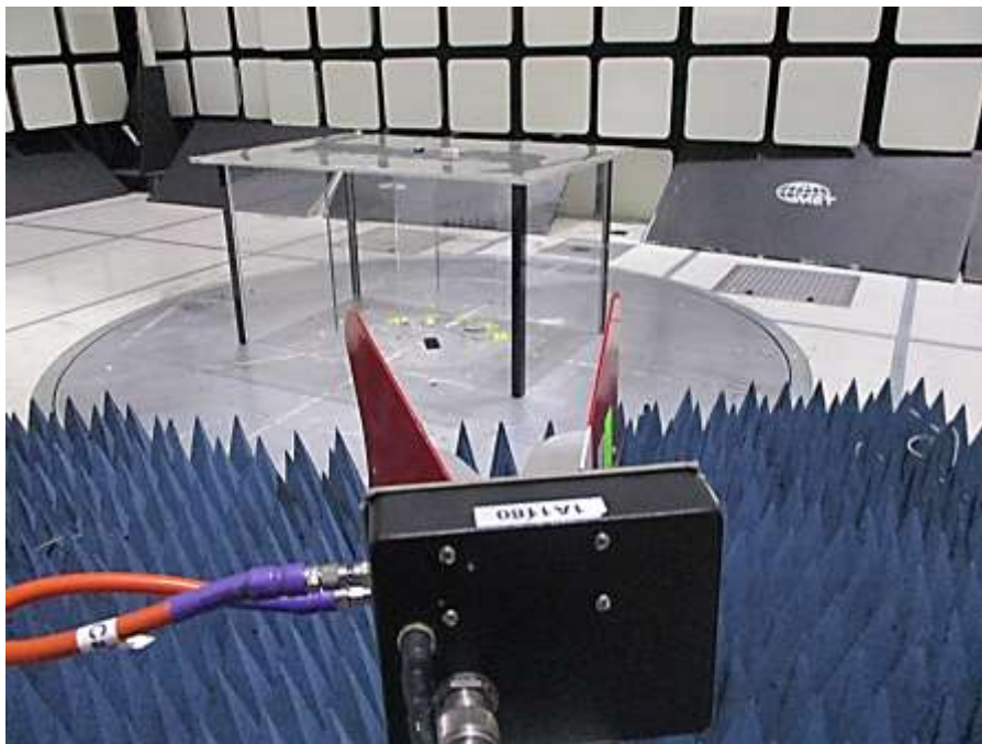
Photograph 6. Radiated Emissions, (1 GHz – 18 GHz), Antenna View
