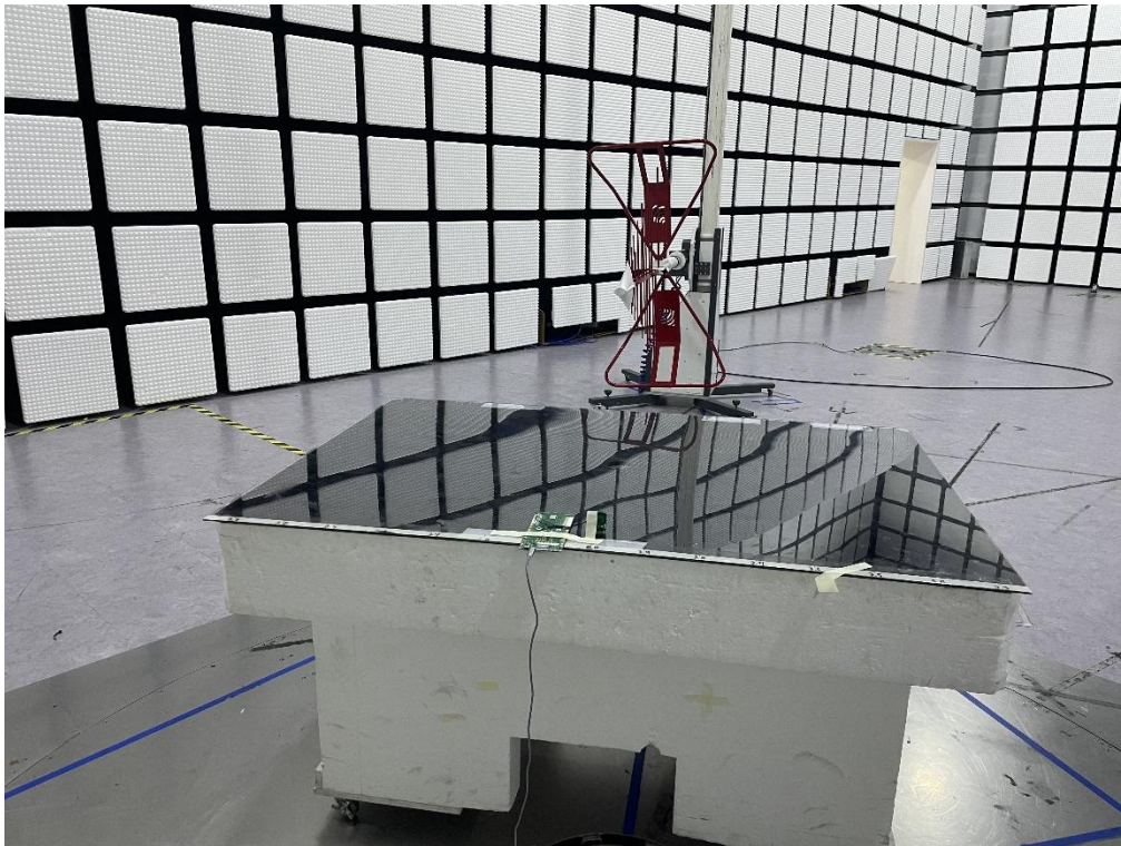
Radiated Emissionss(30MHz ~ 1GHz)
