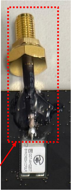
Antenna trace, coaxial cable and Antenna(host) GW.29.A153
