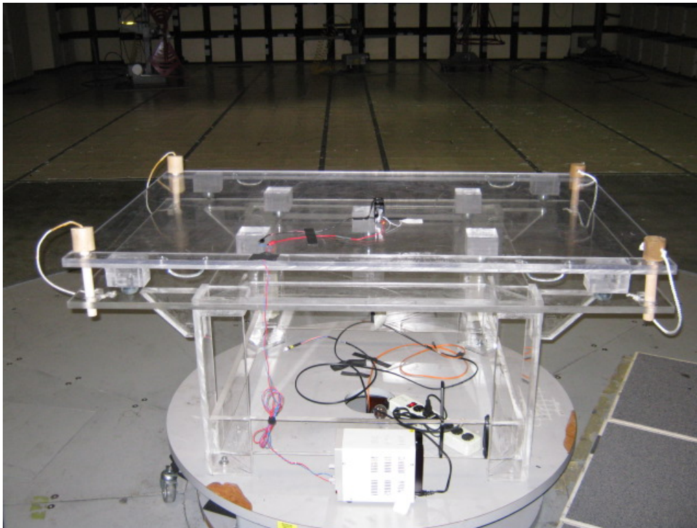
Radiated Emission Spurious 30 MHz to 18 GHz Middle Channel Sample
