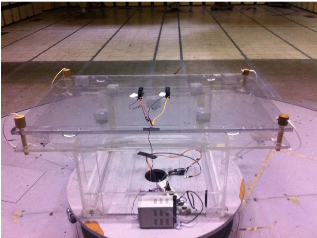
Radiated Emission Spurious 30 MHz to 18 GHz Low & High Channel Samples
