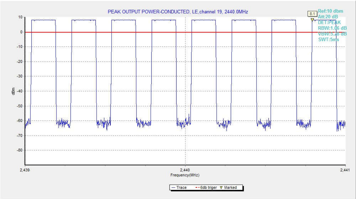
Fig.2 Maximum Peak Output Power(GFSK, Ch 19)
