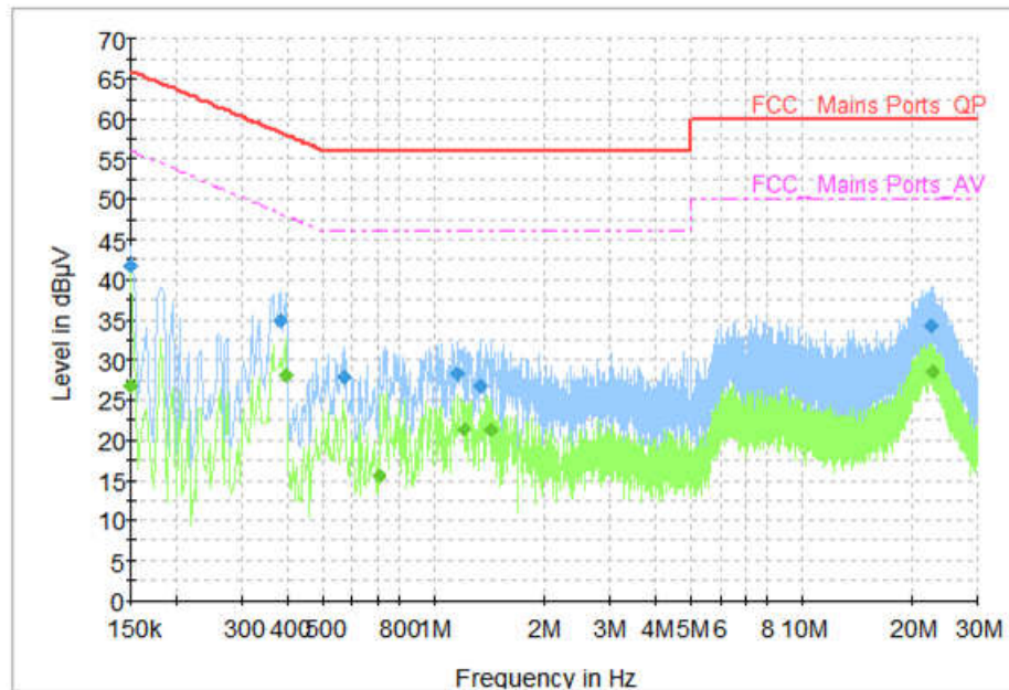
Fig.31 AC Powerline Conducted Emission (Traffic, AE1)
