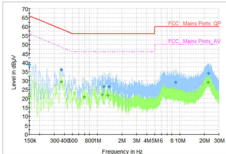
Fig.32 AC Power line Conducted Emission (Idle, AE1)
