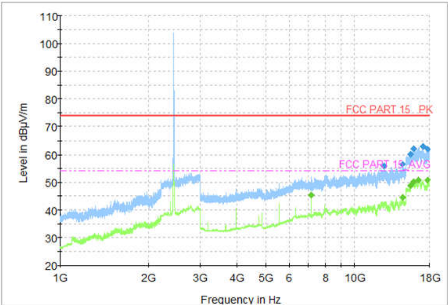
Fig.48 Radiated Spurious Emission (802.11b, CH6, 1 GHz-18GHz)
