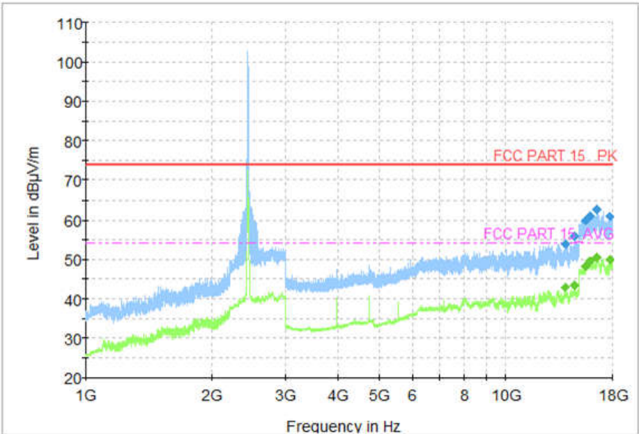
Fig.58 Radiated Spurious Emission (802.11n HT20, CH6, 1 GHz-18 GHz)
