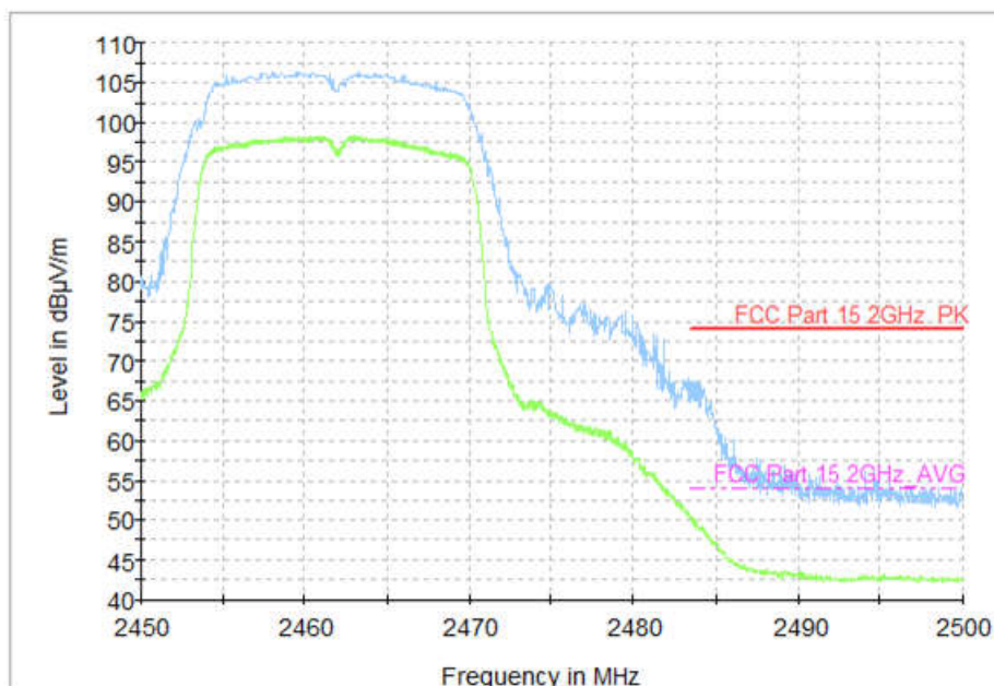
Fig.56 Radiated Restricted Band (802.11g, CH11, 2.45GHz~2.5GHz)
