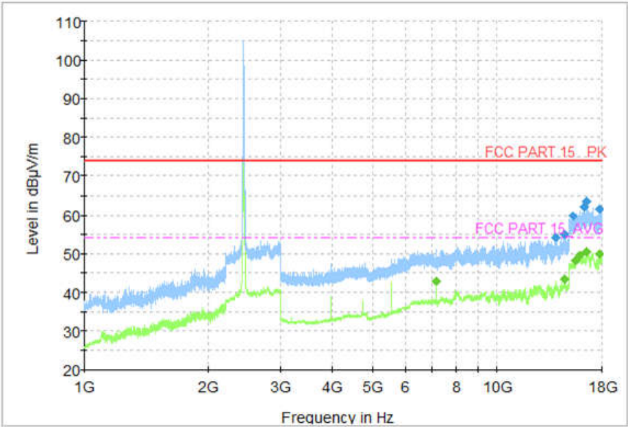
Fig.53 Radiated Spurious Emission (802.11g, CH6, 1 GHz-18 GHz)
