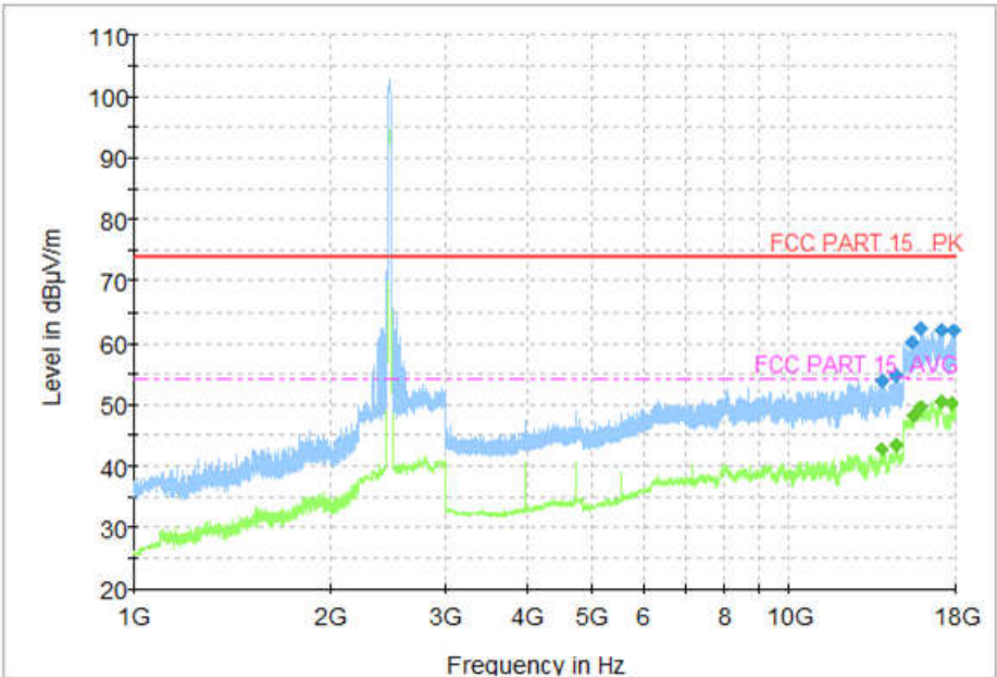
Fig.54 Radiated Spurious Emission (802.11g, CH11, 1 GHz-18 GHz)
