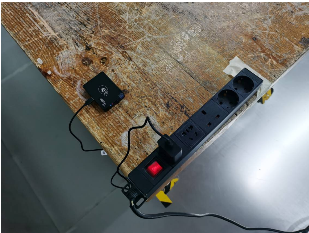
Conducted Emissions Side View-Model: Moby/5500 CL3
