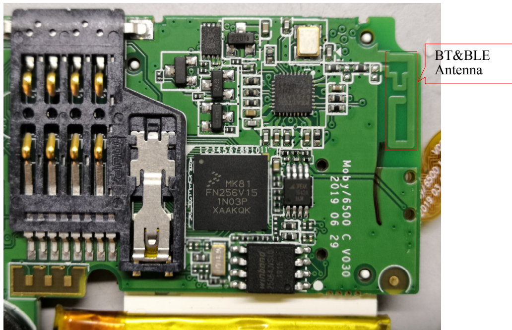
EUT – PCB-2 Chip View-4
