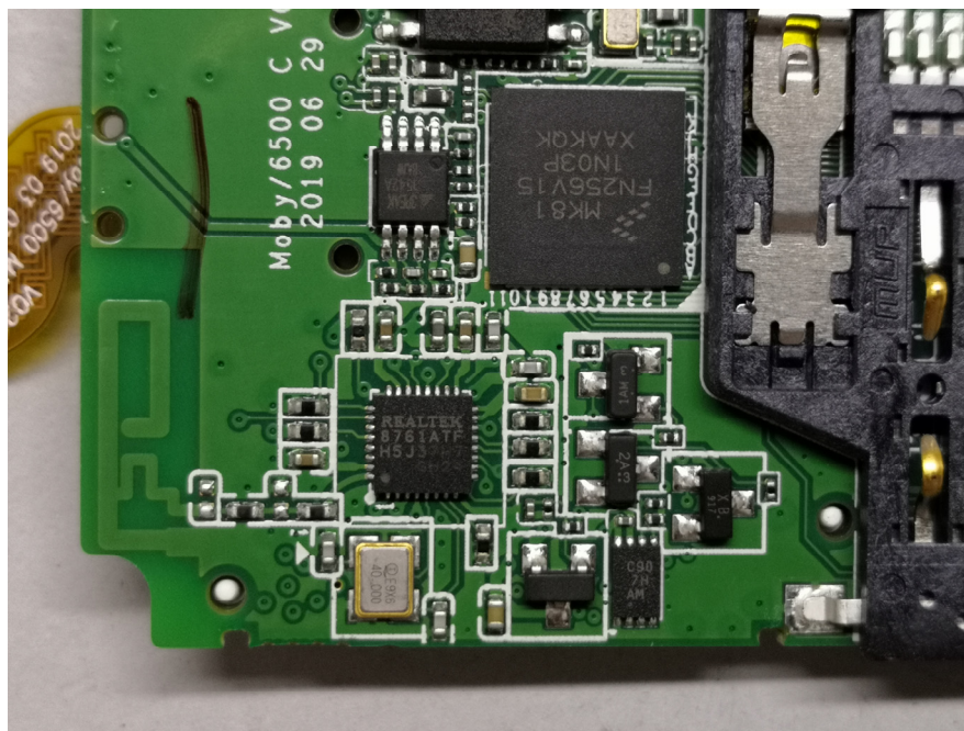
EUT – PCB-2 Chip View-4
