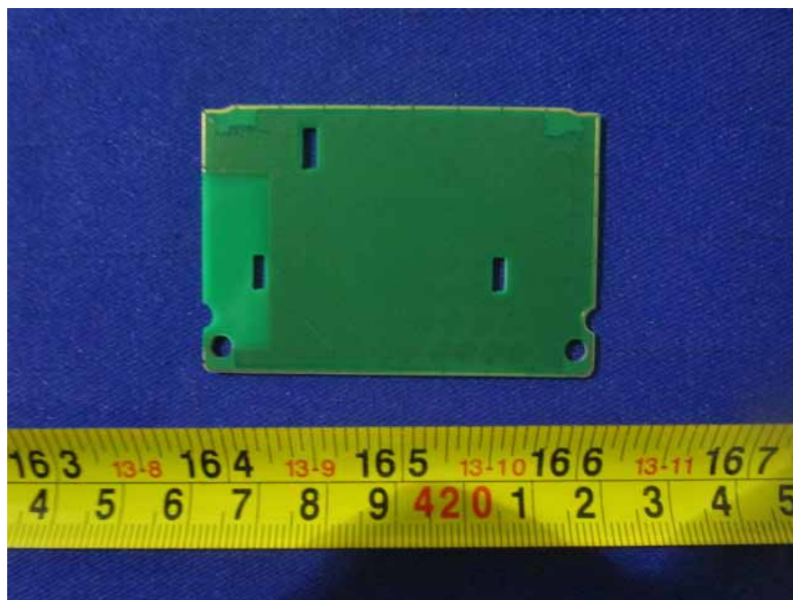
EUT- The Layer of Encryption Board Bottom View
