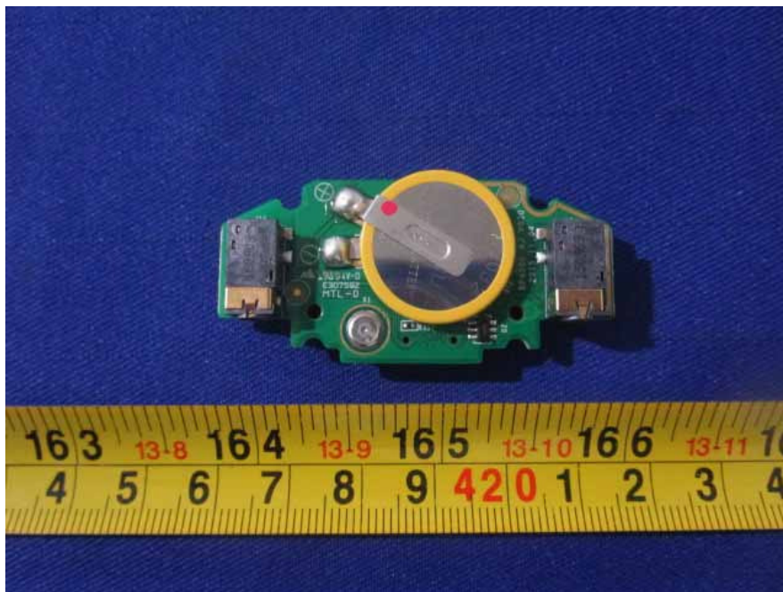
EUT- Audio Input Board Top View
