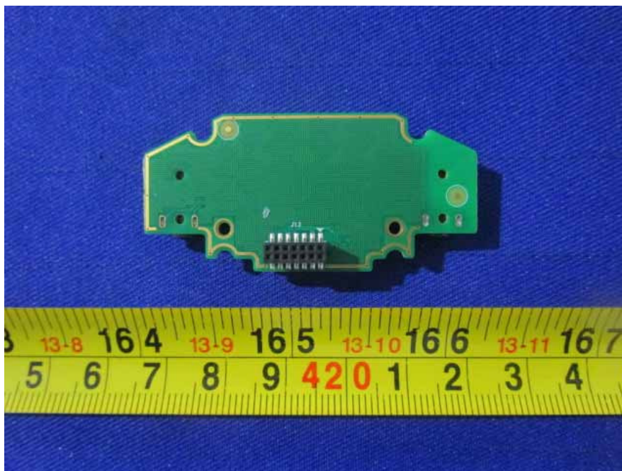
EUT- Audio Input Board Bottom View
