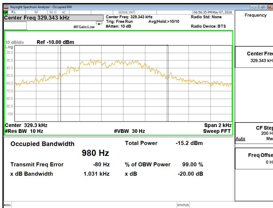
329KHz Coil Antenna 2
