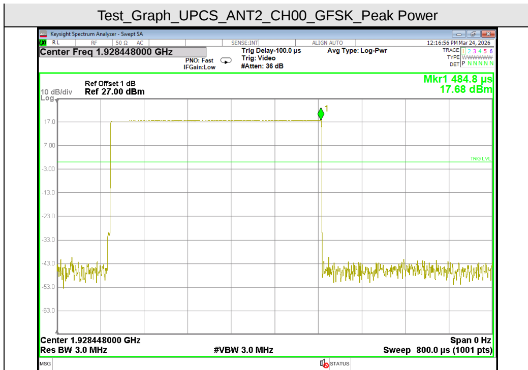
Antenna 2
