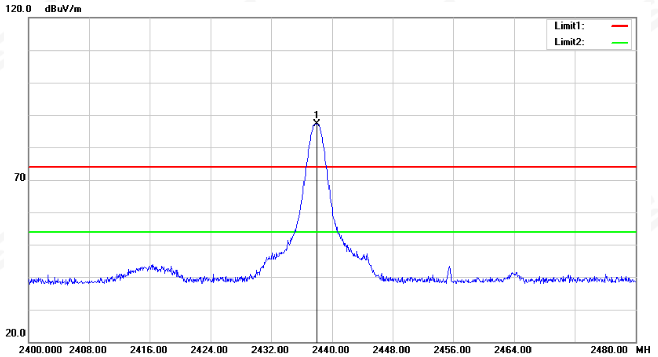
Fundamental Frequency
