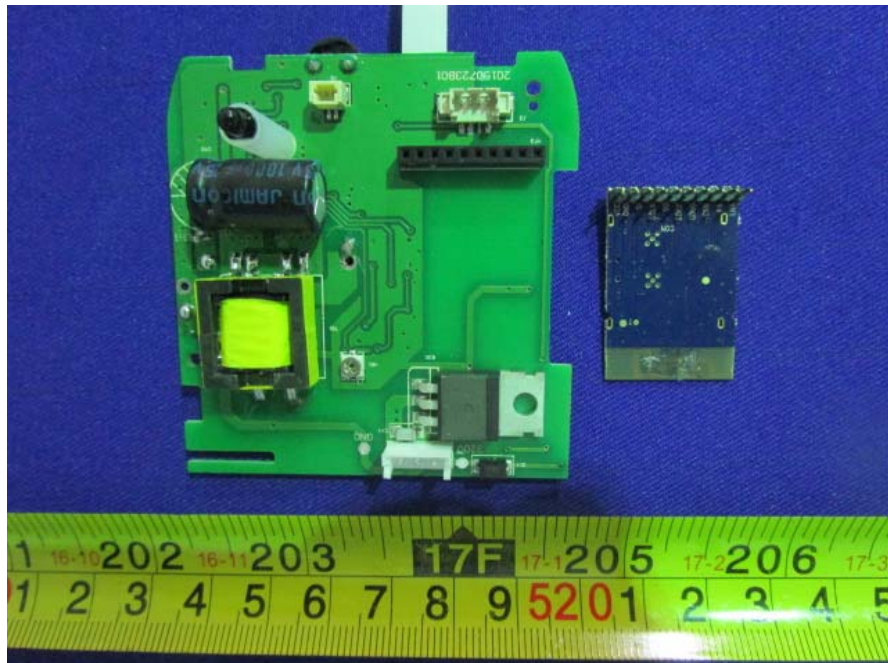
EUT –Power Board Top Uncover View
