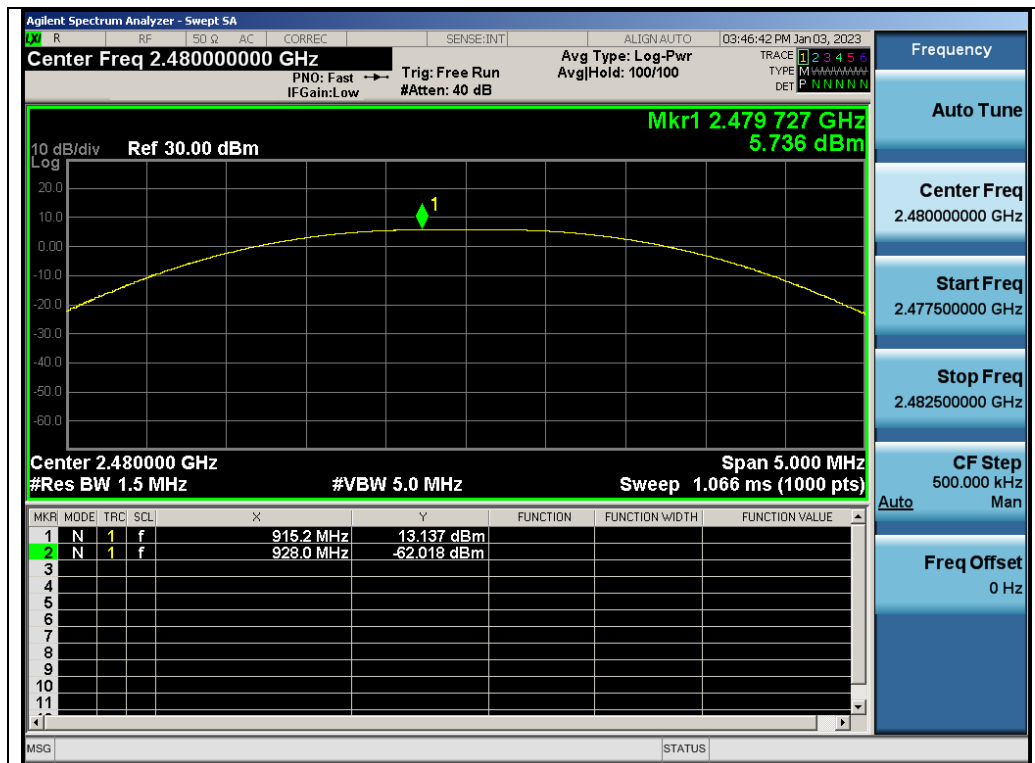
Test_Graph_GFSK_ANT4_2480_125Kbps_Peak Power
