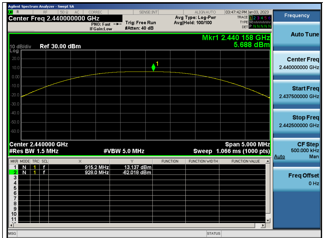
Test_Graph_GFSK_ANT4_2440_500Kbps_Peak Power
