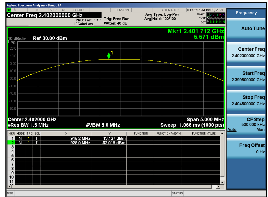
Test_Graph_GFSK_ANT4_2402_125Kbps_Peak Power
