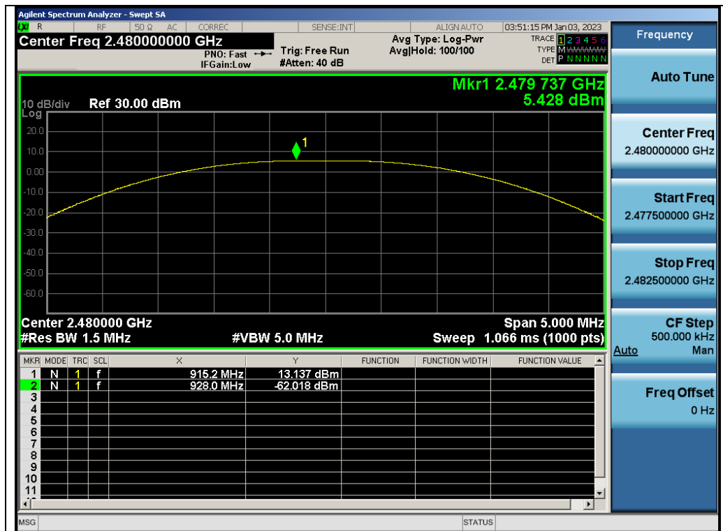
Test_Graph_GFSK_ANT5_2480_125Kbps_Peak Power
