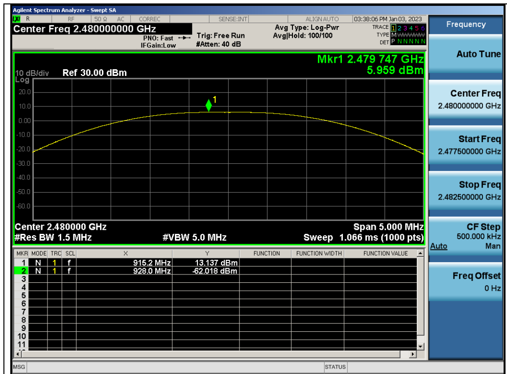
Test_Graph_GFSK_ANT3_2480_125Kbps_Peak Power
