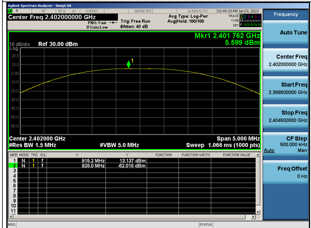
Test_Graph_GFSK_ANT5_2402_500Kbps_Peak Power
