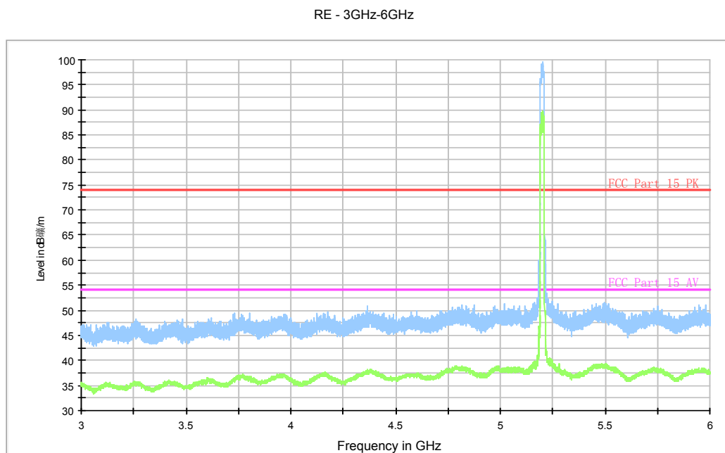
Fig. 41 Radiated Spurious Emission (802.11n-HT20, ch40, 3 GHz-6 GHz)
