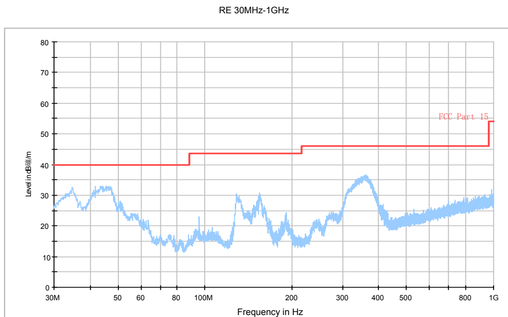
Fig. 39 Radiated Spurious Emission (802.11n-HT20, ch40, 30 MHz-1 GHz)
