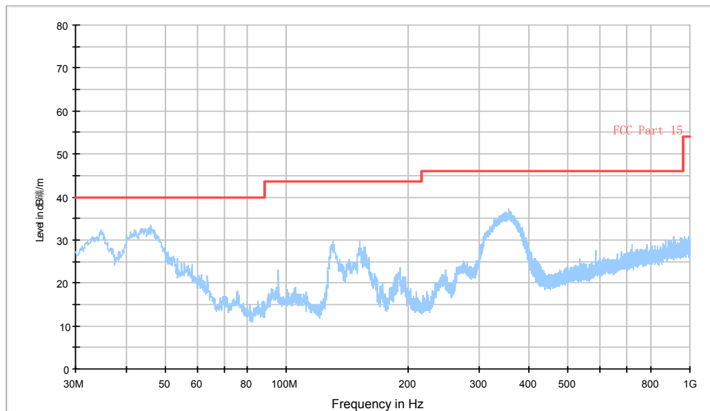
Fig. 27 Radiated Spurious Emission (802.11a, ch40, 30 MHz-1 GHz)
