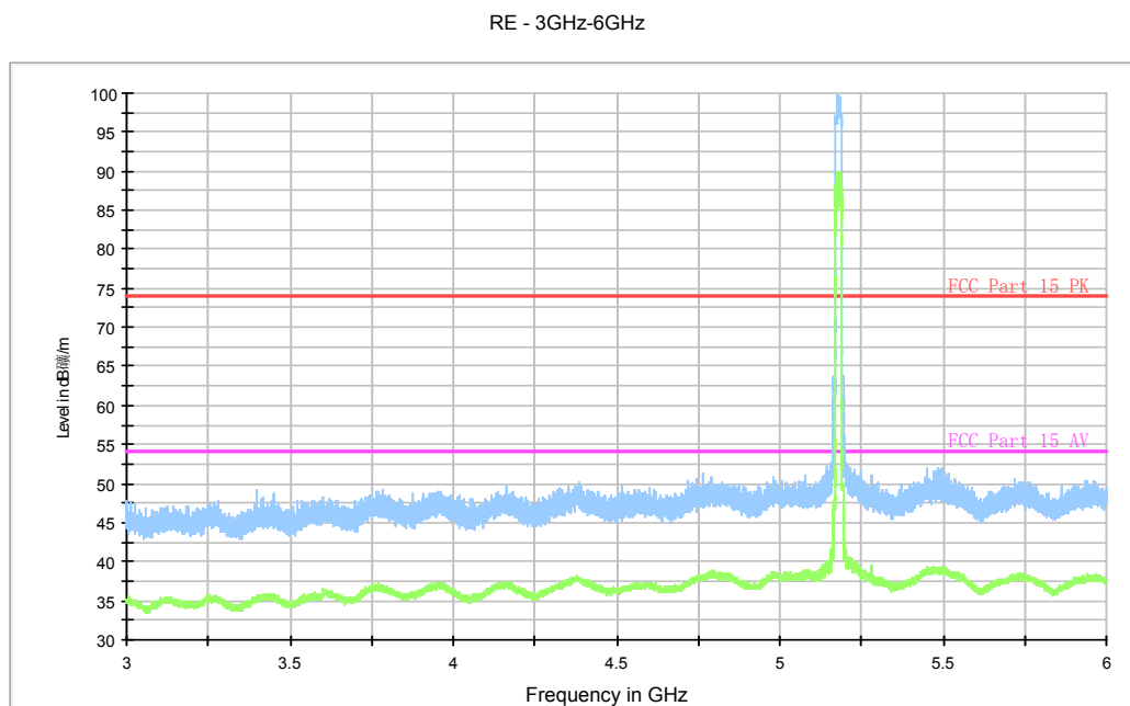
Fig. 37 Radiated Spurious Emission (802.11n-HT20, ch36, 3 GHz-6 GHz)
