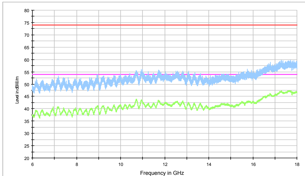
Fig. 30 Radiated Spurious Emission (802.11a, ch40, 6 GHz-18 GHz)
