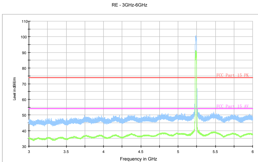
Fig. 34 Radiated Spurious Emission (802.11a, ch48, 3 GHz-6 GHz)
