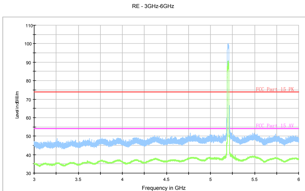
Fig. 29 Radiated Spurious Emission (802.11a, ch40, 3 GHz-6 GHz)
