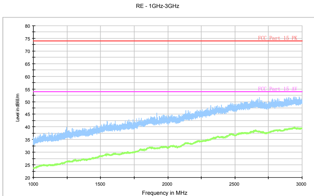
Fig. 36 Radiated Spurious Emission (802.11n-HT20, ch36, 1 GHz-3 GHz)
