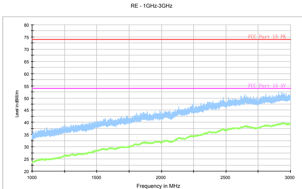
Fig. 40 Radiated Spurious Emission (802.11n-HT20, ch40, 1 GHz-3 GHz)
