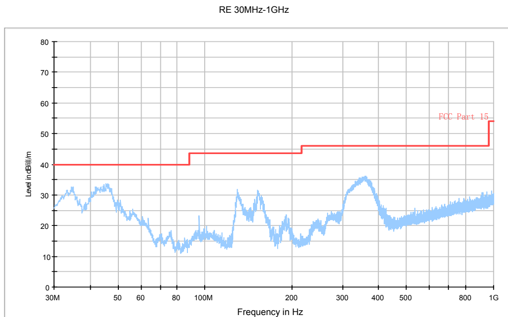
Fig. 48 Radiated Spurious Emission (802.11n-HT40, ch38, 30 MHz-1 GHz)
