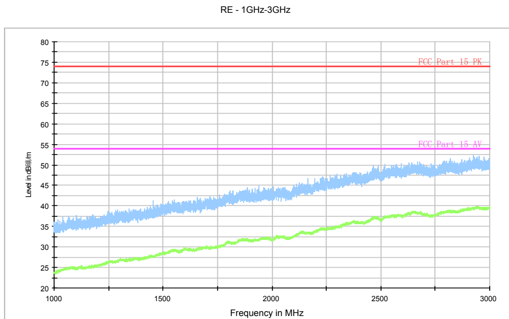
Fig. 28 Radiated Spurious Emission (802.11a, ch40, 1 GHz-3 GHz)
