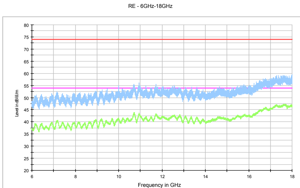
Fig. 47 Radiated Spurious Emission (802.11n-HT20, ch48, 6 GHz-18 GHz)
