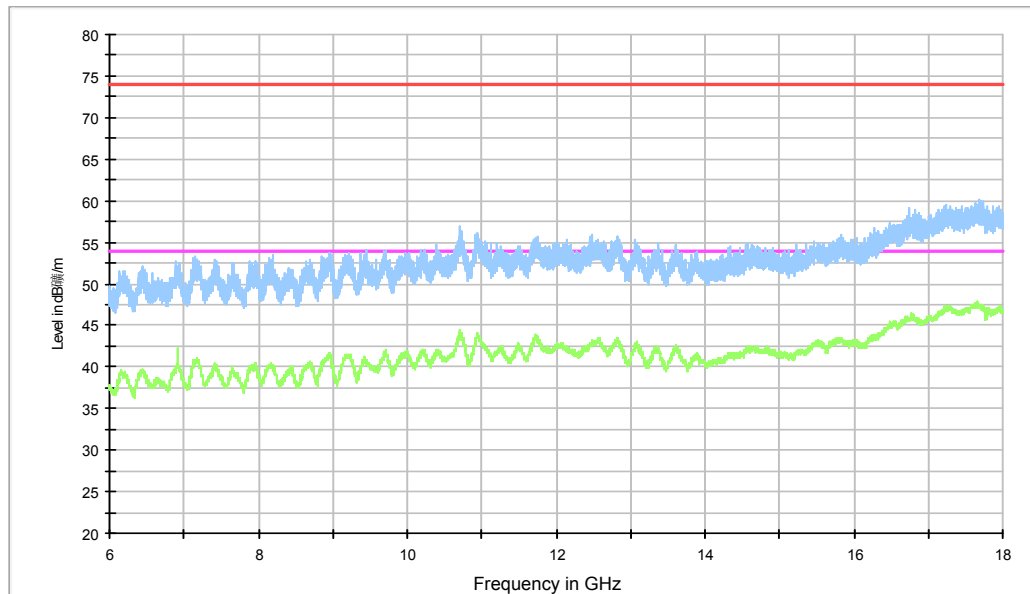
Fig. 26 Radiated Spurious Emission (802.11a, ch36, 6 GHz-18 GHz)
