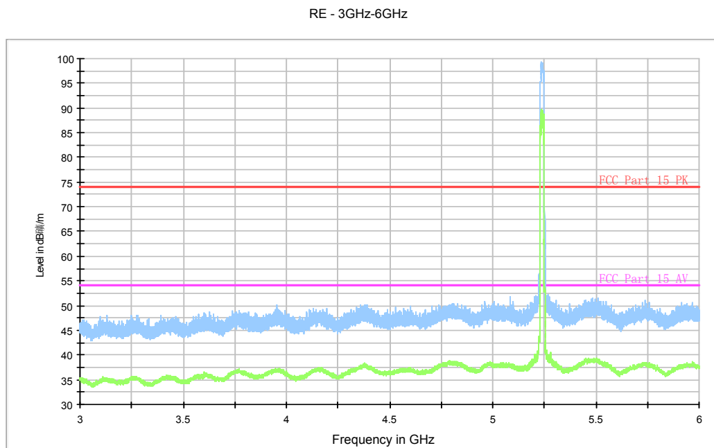
Fig. 46 Radiated Spurious Emission (802.11n-HT20, ch48, 3 GHz-6GHz)
