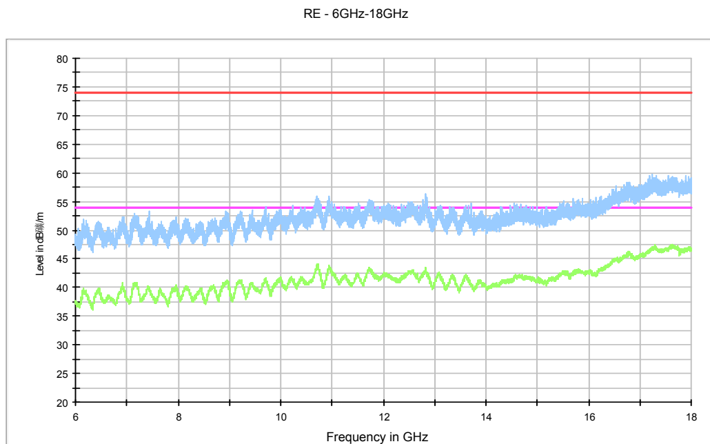
Fig. 38 Radiated Spurious Emission (802.11n-HT20, ch36, 6 GHz-18GHz)
