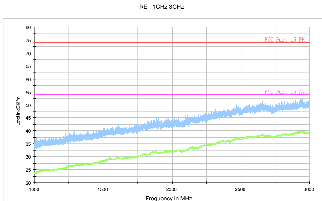
Fig. 49 Radiated Spurious Emission (802.11n-HT40, ch38, 1 GHz-3 GHz)
