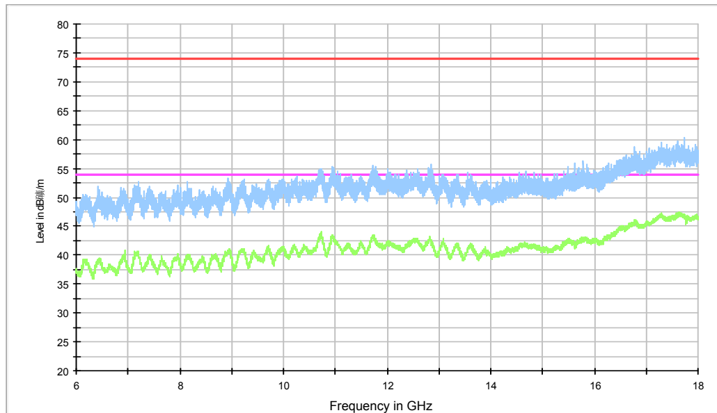
Fig. 42 Radiated Spurious Emission (802.11n-HT20, ch40, 6 GHz-18 GHz)
